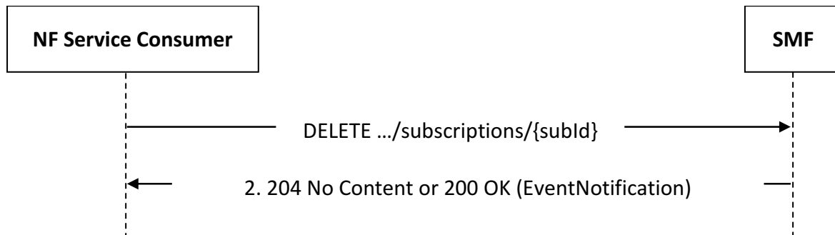
Figure 4.2.4.2-1: Unsubscription from event notifications
