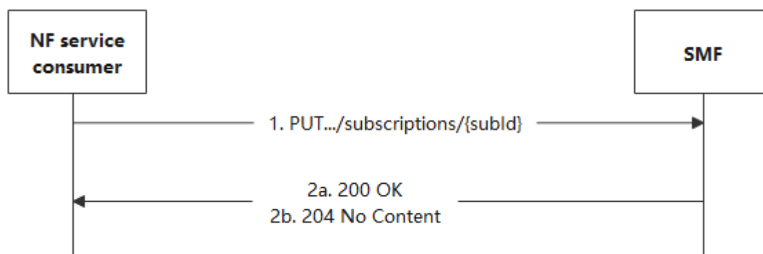
Figure 4.2.3.3-1: Modification of an existing subscription
