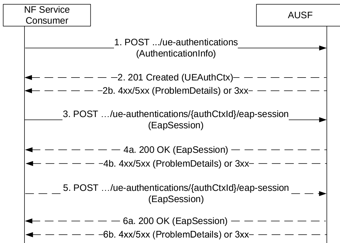
Figure 5.2.2.2.3-1: EAP-based authentication with EAP-AKA' method
