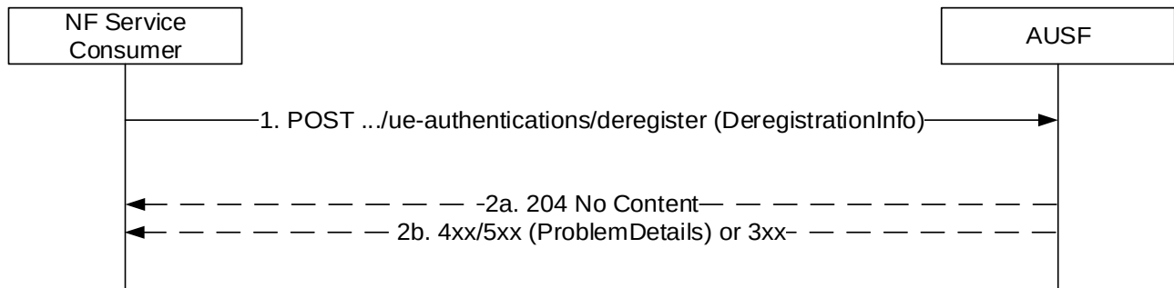
Figure 5.2.2.3.1-1: UE Context Clean-up in AUSF
