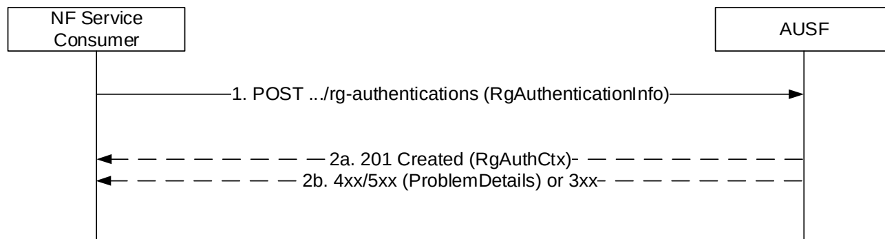
Figure 5.2.2.2.4-1: Authentication for FN-RG
