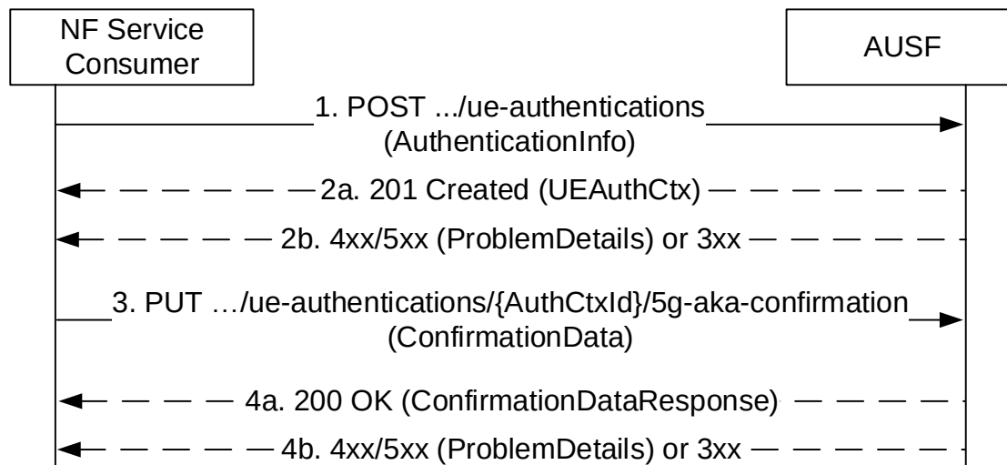
Figure 5.2.2.2-1: 5G AKA
