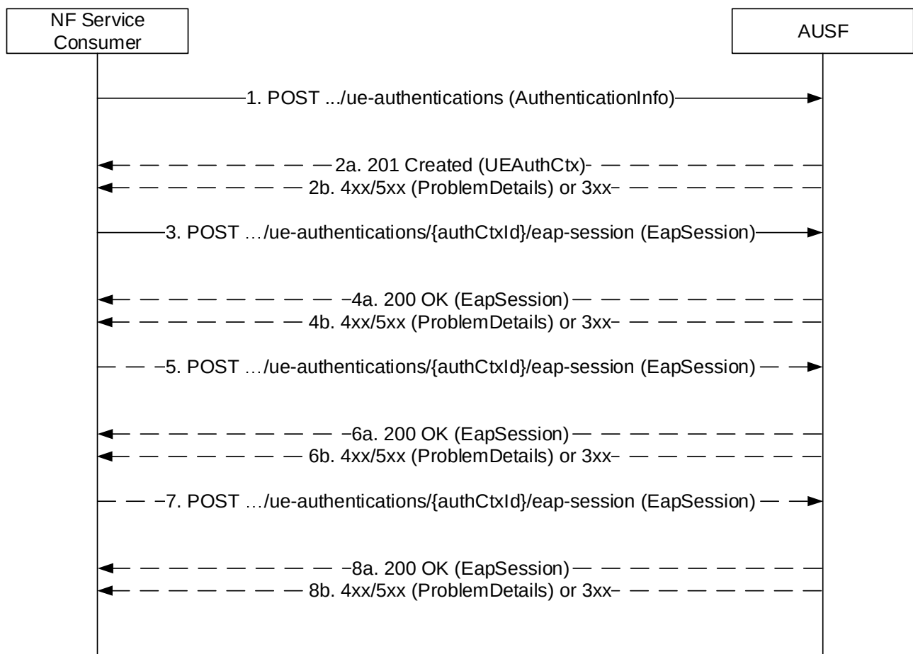
Figure B.2-1: EAP method
