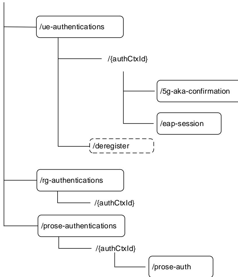
Figure 6.1.3.1-1: Resource URI structure of the AUSF API
