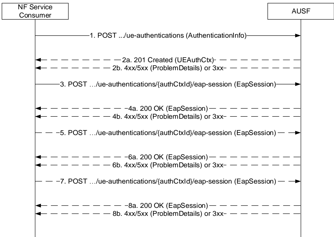
Figure B.2-1: EAP method
