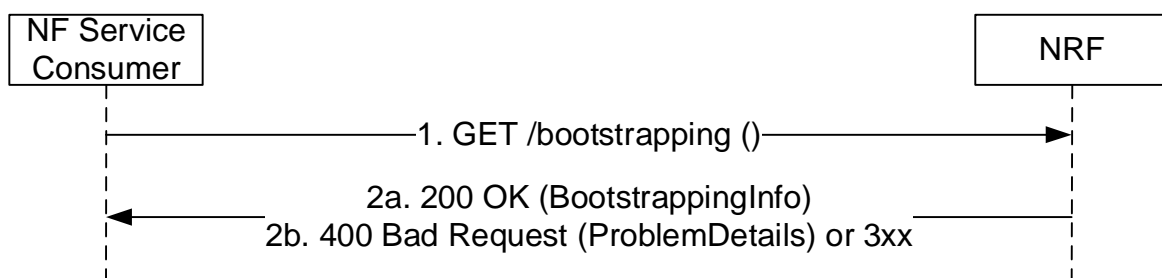
Figure 5.5.2.2.1-1: Bootstrapping Request
