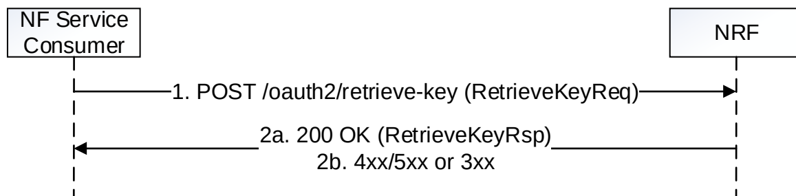
Figure 5.4.2.3.1-1: Access Token Request
