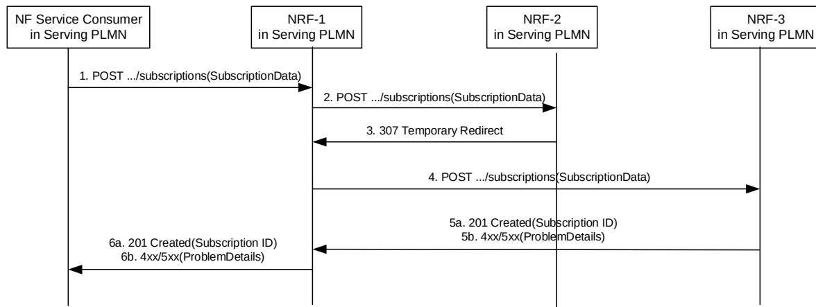
Figure 5.2.2.5.5-1: Subscription to NF Instances with intermediate redirecting NRF
