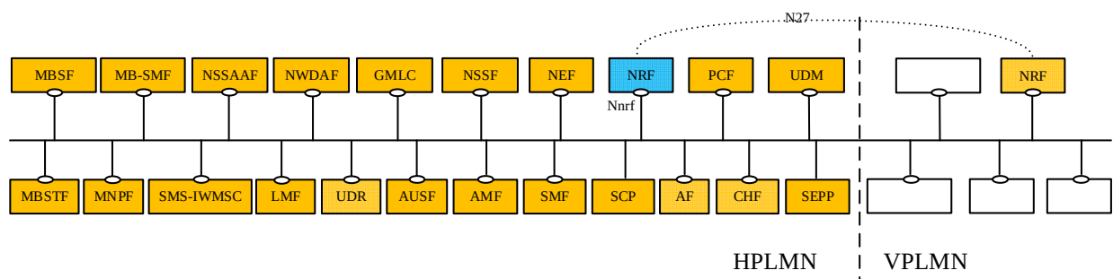
Figure 4-1: 5G System architecture
