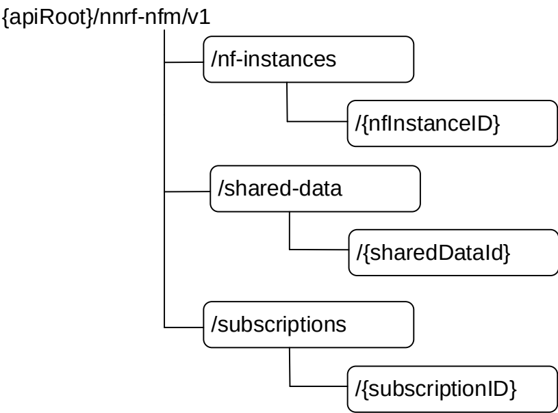
Figure 6.1.3.1-1: Resource URI structure of the NFManagement API
