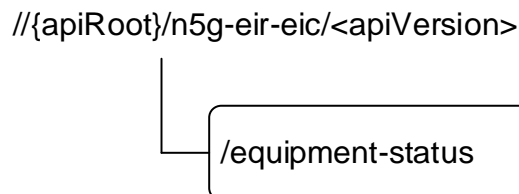
Figure 6.1.3.1-1: Resource URI structure of the n5g-eir-eic API
