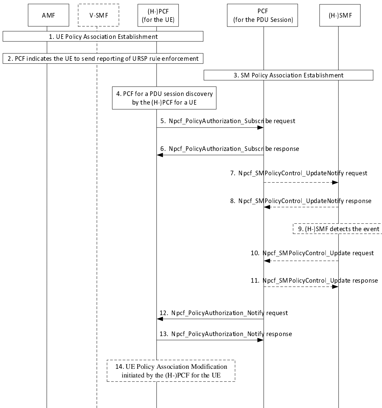
Figure 5.8.2-1: Forwarding of URSP Rule Enforcement Information (non-roaming and Home Routed roaming)
