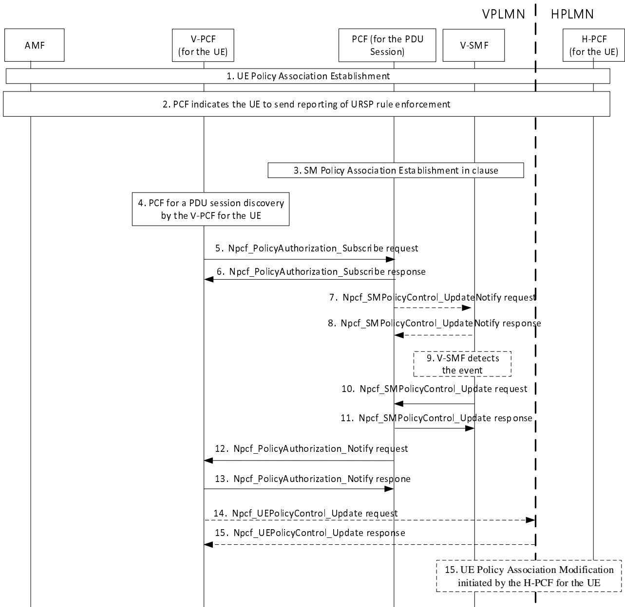
Figure 5.8.3-1: Forwarding of URSP Rule Enforcement Information (LBO roaming)
