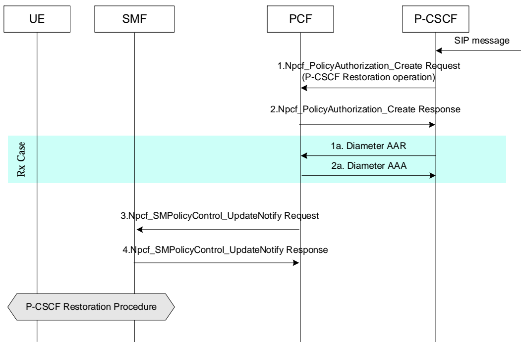
Figure B.9-1: P-CSCF Restoration
