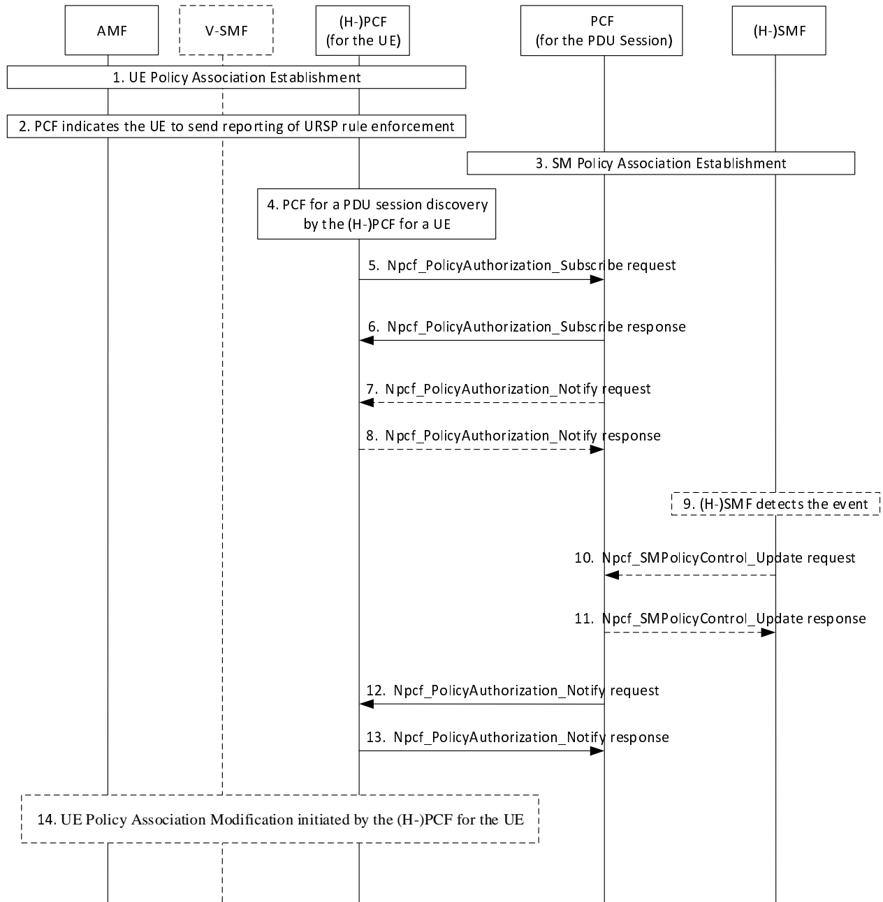
Figure 5.8.2-1: Forwarding of URSP Rule Enforcement Information (non-roaming and Home Routed roaming)
