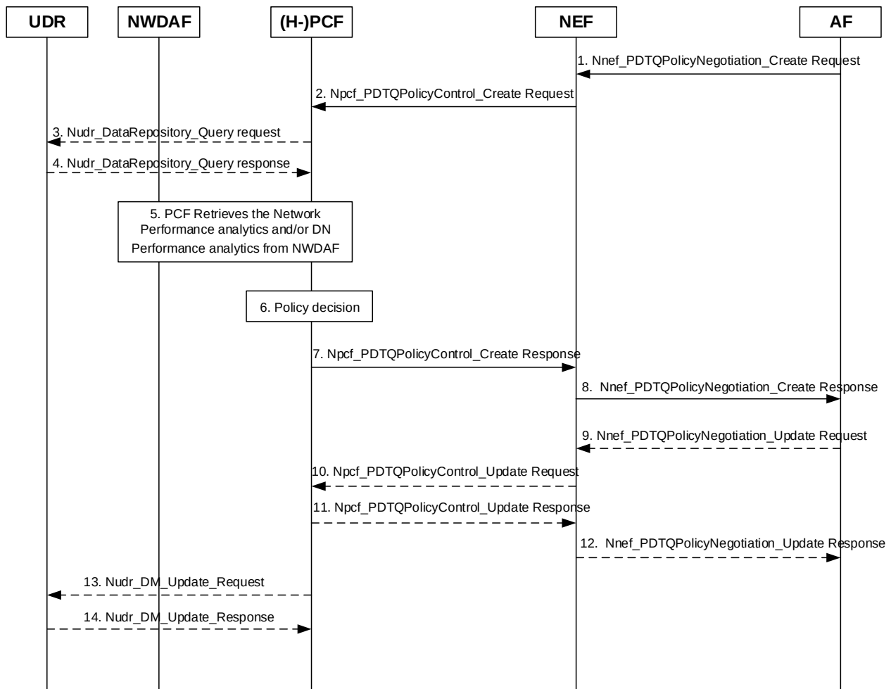
Figure 5.5.13-1: Negotiation for PDTQ procedure
