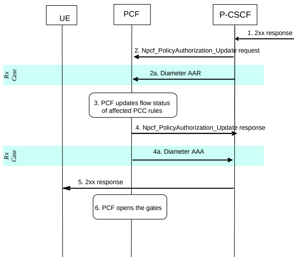
Figure B.3.2-1: Enabling of IP Flows
