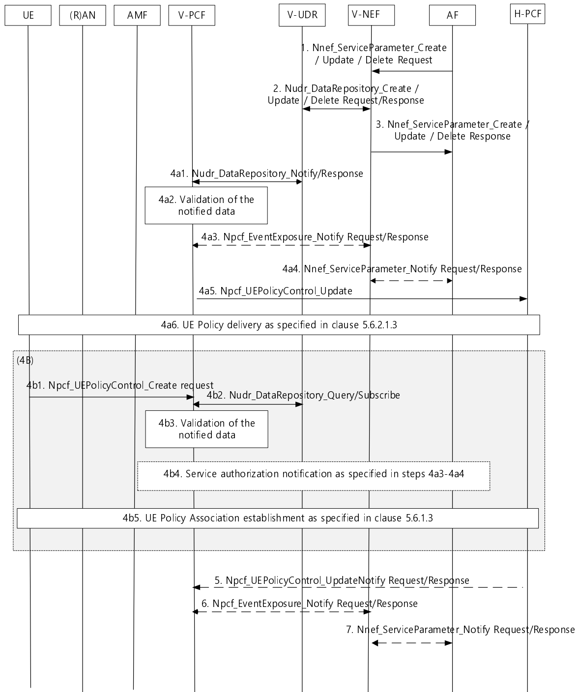
Figure 5.5.8.2-1: AF-based service parameter provisioning procedure to VPLMN
