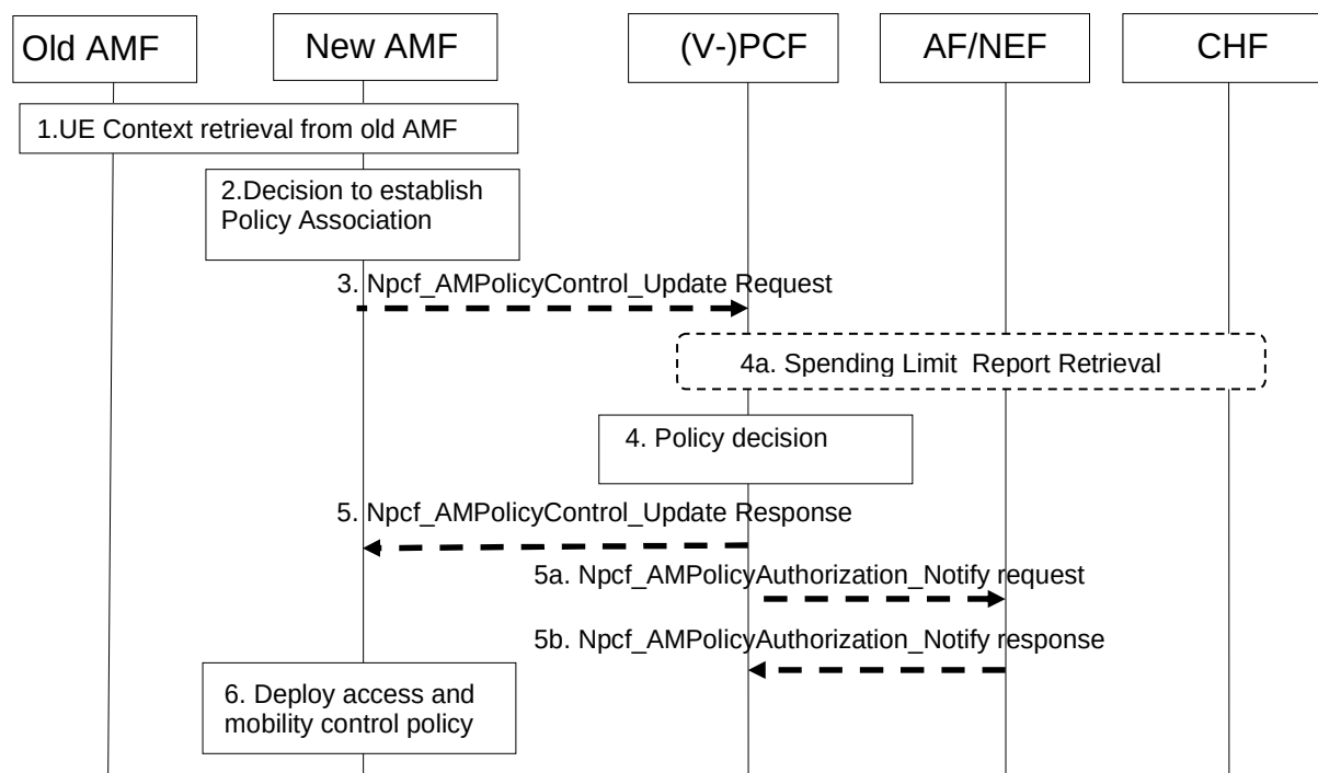
Figure 5.1.2.1.2-1: AMF-initiated AM Policy Association Modification with old PCF during AMF relocation procedure
