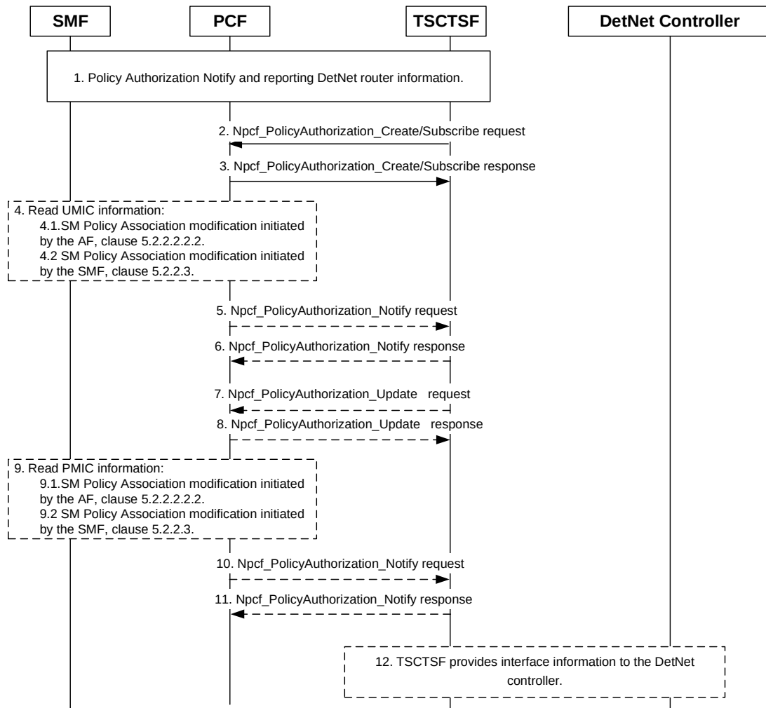
Figure 5.5.12.2-1: 5GS DetNet node information reporting
