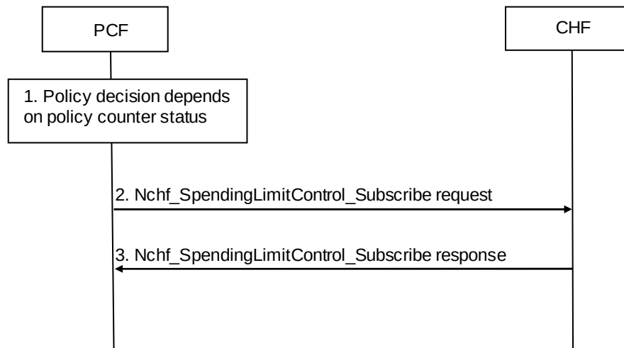
Figure 5.3.2-1: Initial Spending Limit Report Request procedure
