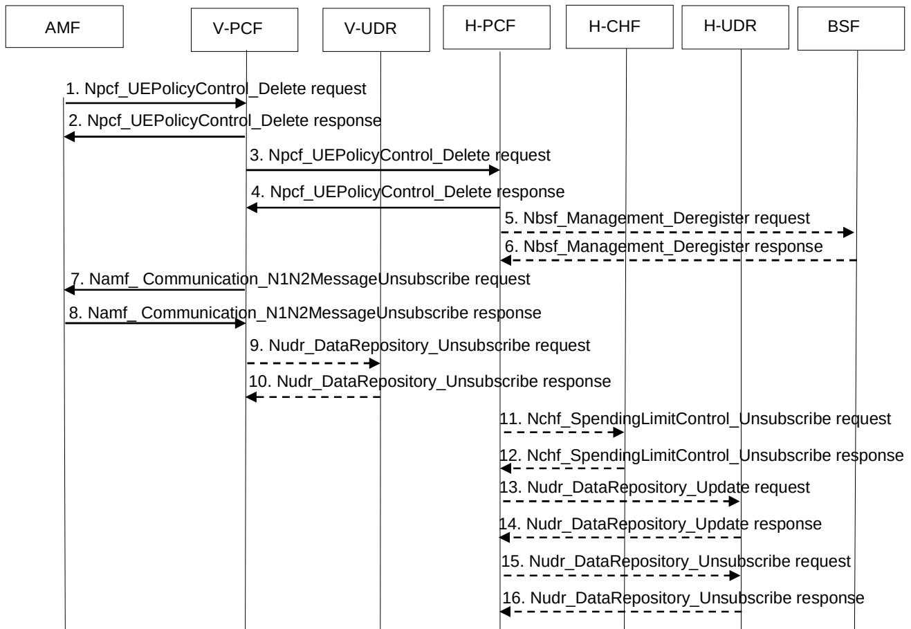
Figure 5.6.3.1.3-1: AMF-initiated UE Policy Association Termination procedure – Roaming
