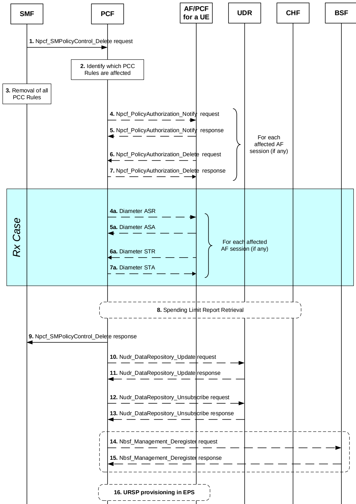
Figure 5.2.3.1-1: SMF-initiated SM Policy Association Termination procedure
