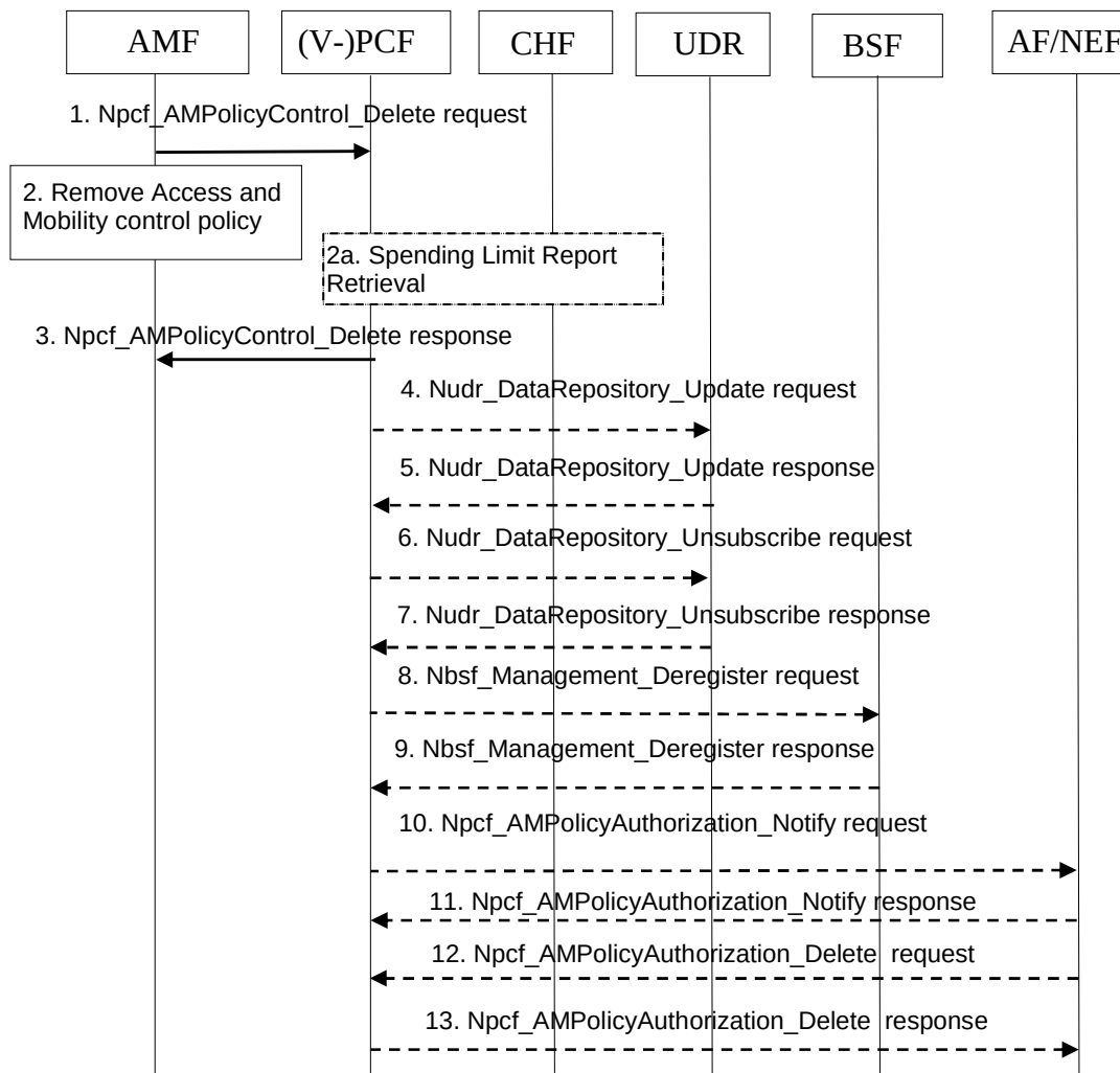
Figure 5.1.3.1-1: AMF-initiated AM Policy Association Termination procedure
