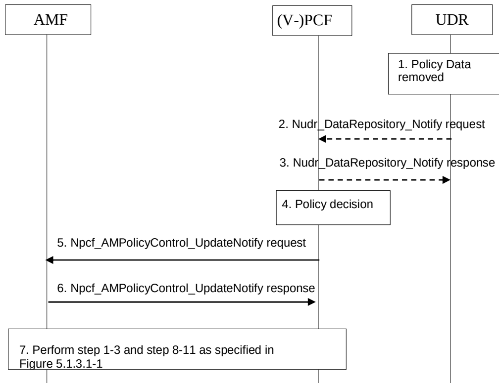
Figure 5.1.3.2-1: PCF-initiated AM Policy Association Termination procedure
