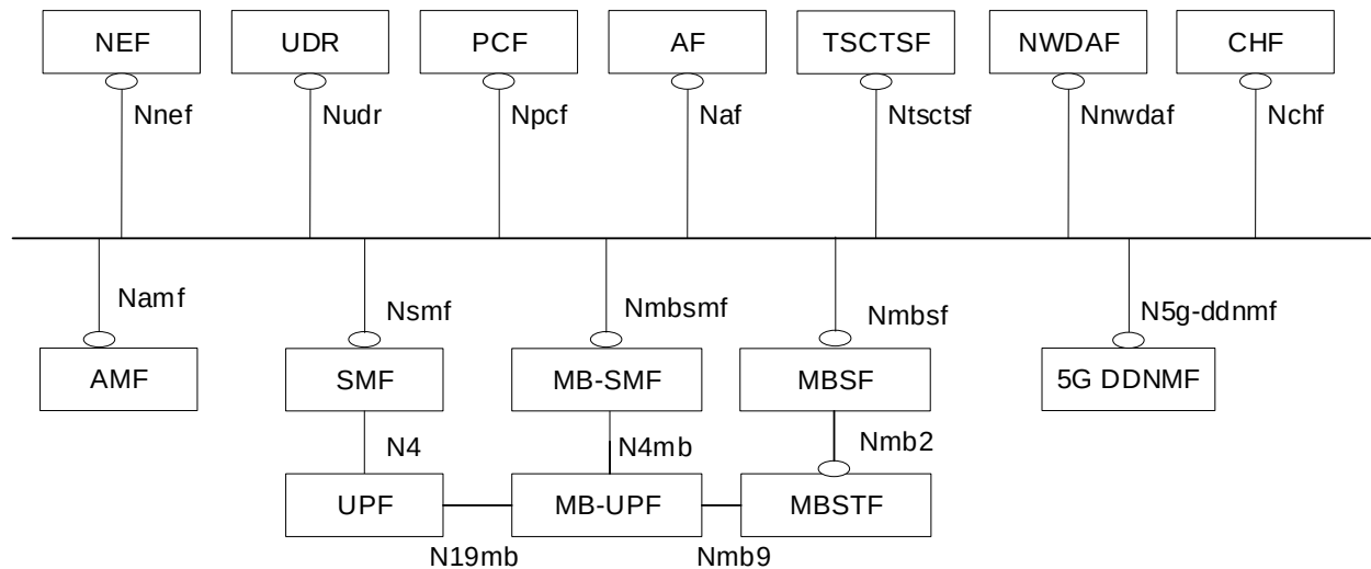
Figure 4.1-1a: Overall non-roaming 5G Policy framework architecture (service based representation)
