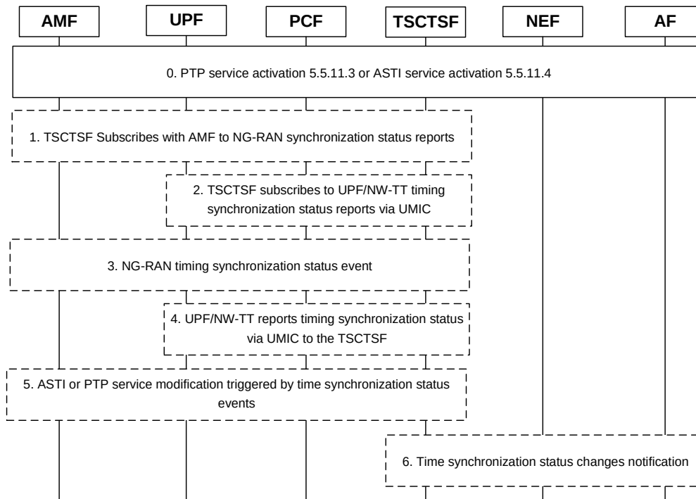
Figure 5.5.11.5-1: Management of network timing synchronization status monitoring
