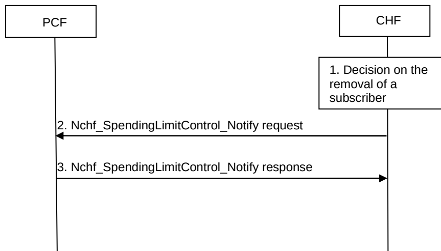
Figure 5.3.6-1: Subscription Termination Request procedure
