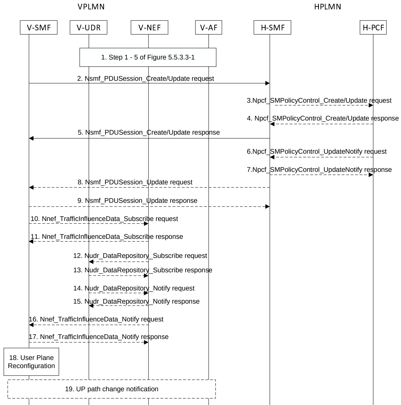
Figure 5.5.3.4-1: Processing AF requests on PDU Sessions supporting HR-SBO
