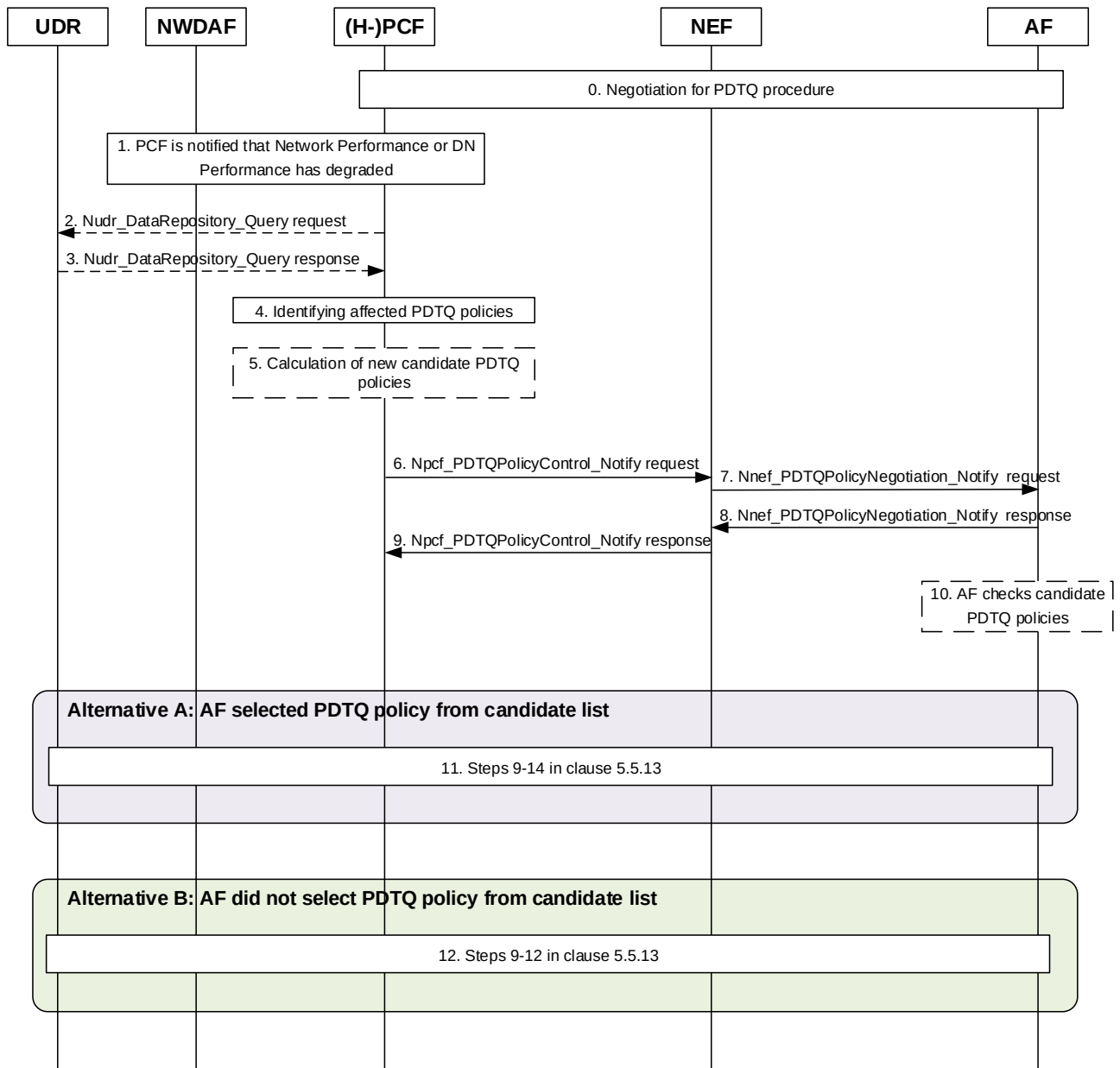
Figure 5.5.14-1: PDTQ warning notification procedure
