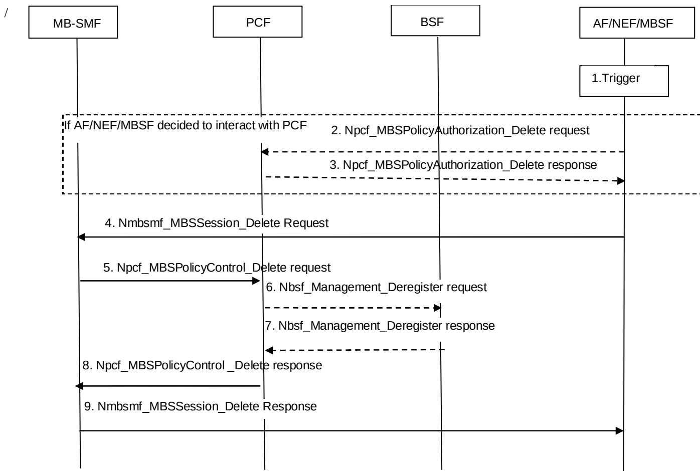
Figure 5.7.4.3-1: MBS Policy Association termination procedure initiated by the AF.
