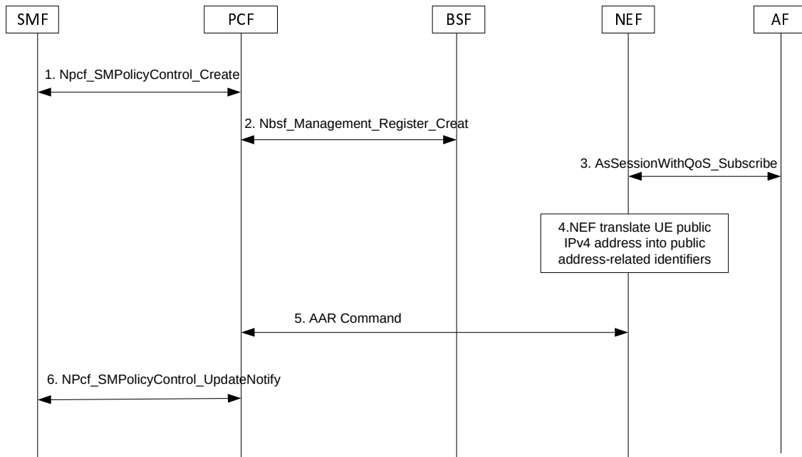
Figure D.2-2: NEF translate public IPv4 address to public address-related identifier in IP domain in Rx interface
