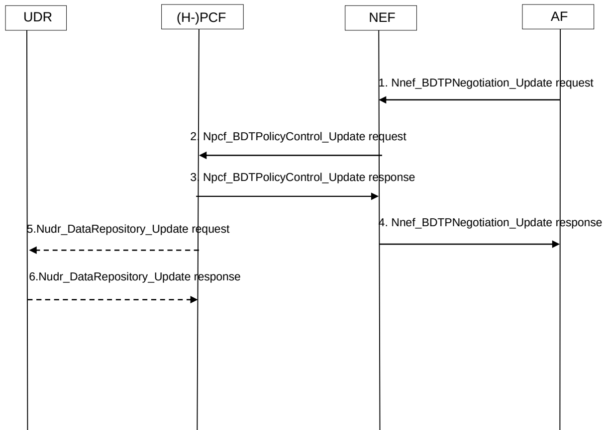
Figure 5.5.4A-1: Modification of BDT warning notification request indication procedure
