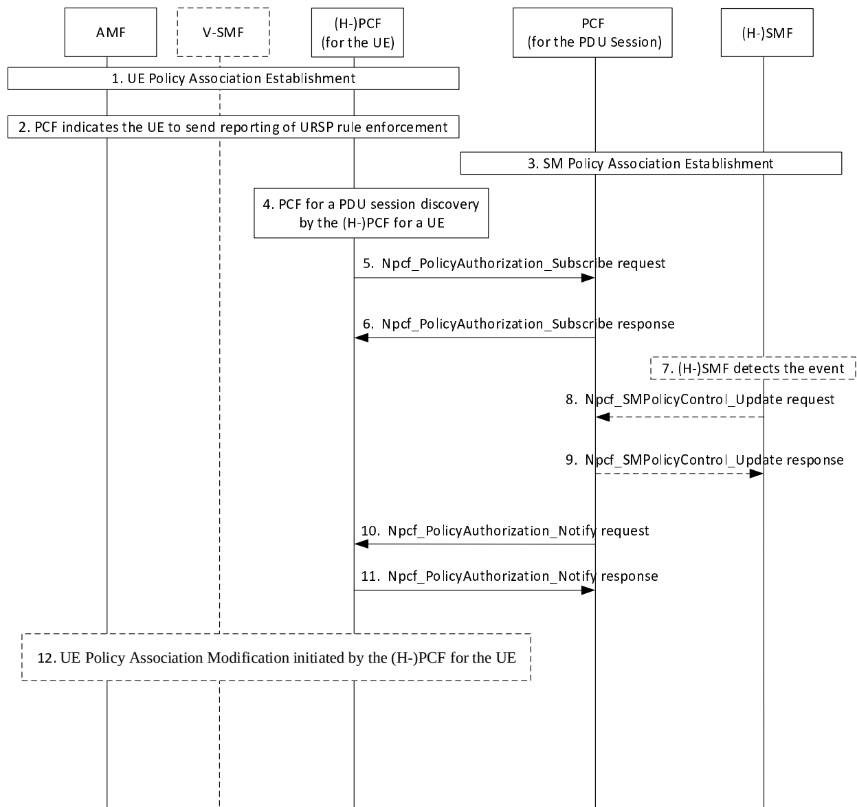
Figure 5.8.2-1: Forwarding of URSP Rule Enforcement Information (non-roaming and Home Routed roaming)
