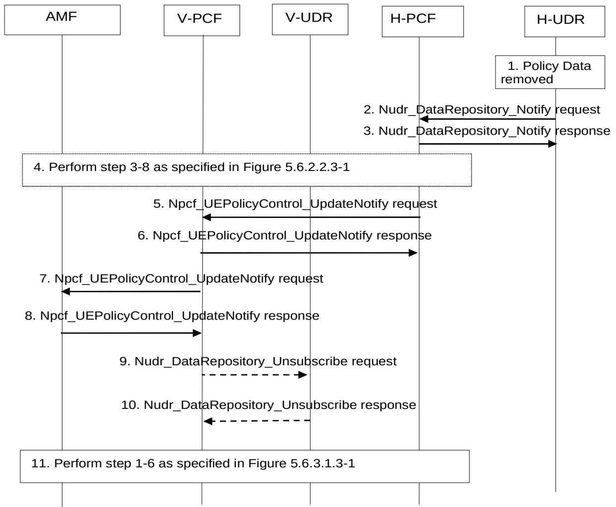
Figure 5.6.3.2.3-1: PCF-initiated UE Policy Association Termination procedure – Roaming
