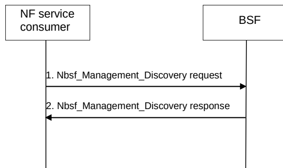
Figure 8.5.4-1: Binding information Retrieval procedure
