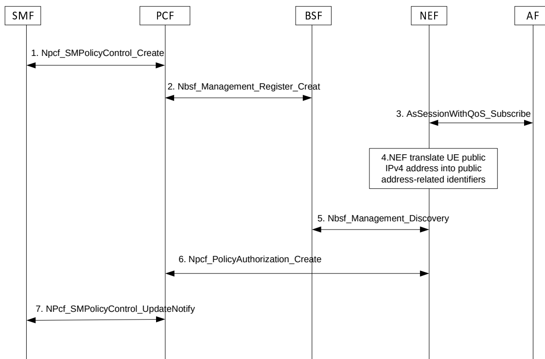
Figure D.2-1: NEF translate public IPv4 address to public address-related identifier in IP domain in N5 interface
