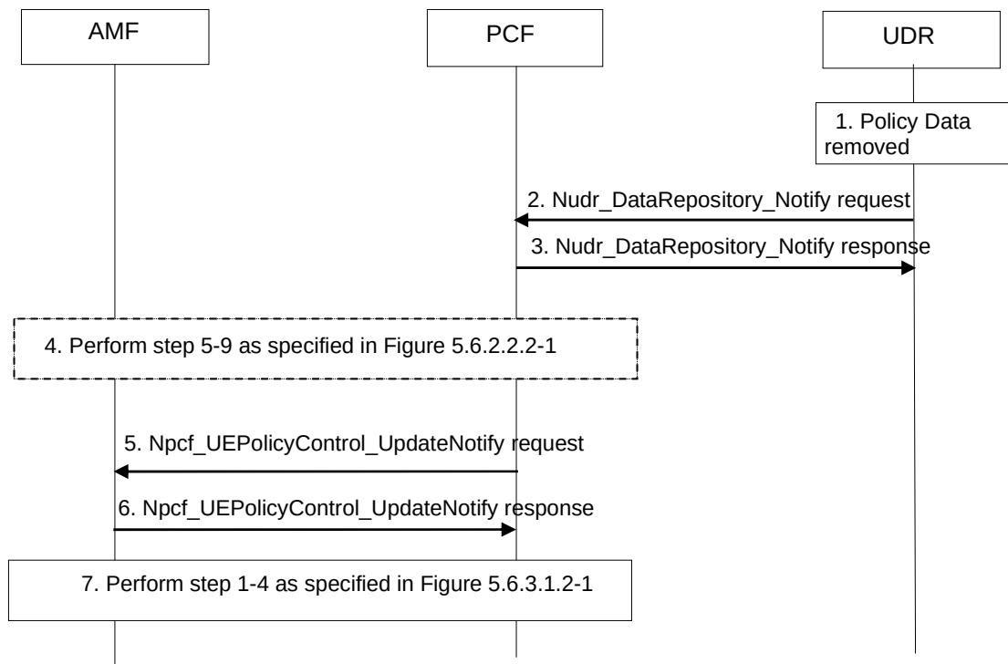
Figure 5.6.3.2.2-1: PCF-initiated UE Policy Association Termination procedure – Non-roaming
