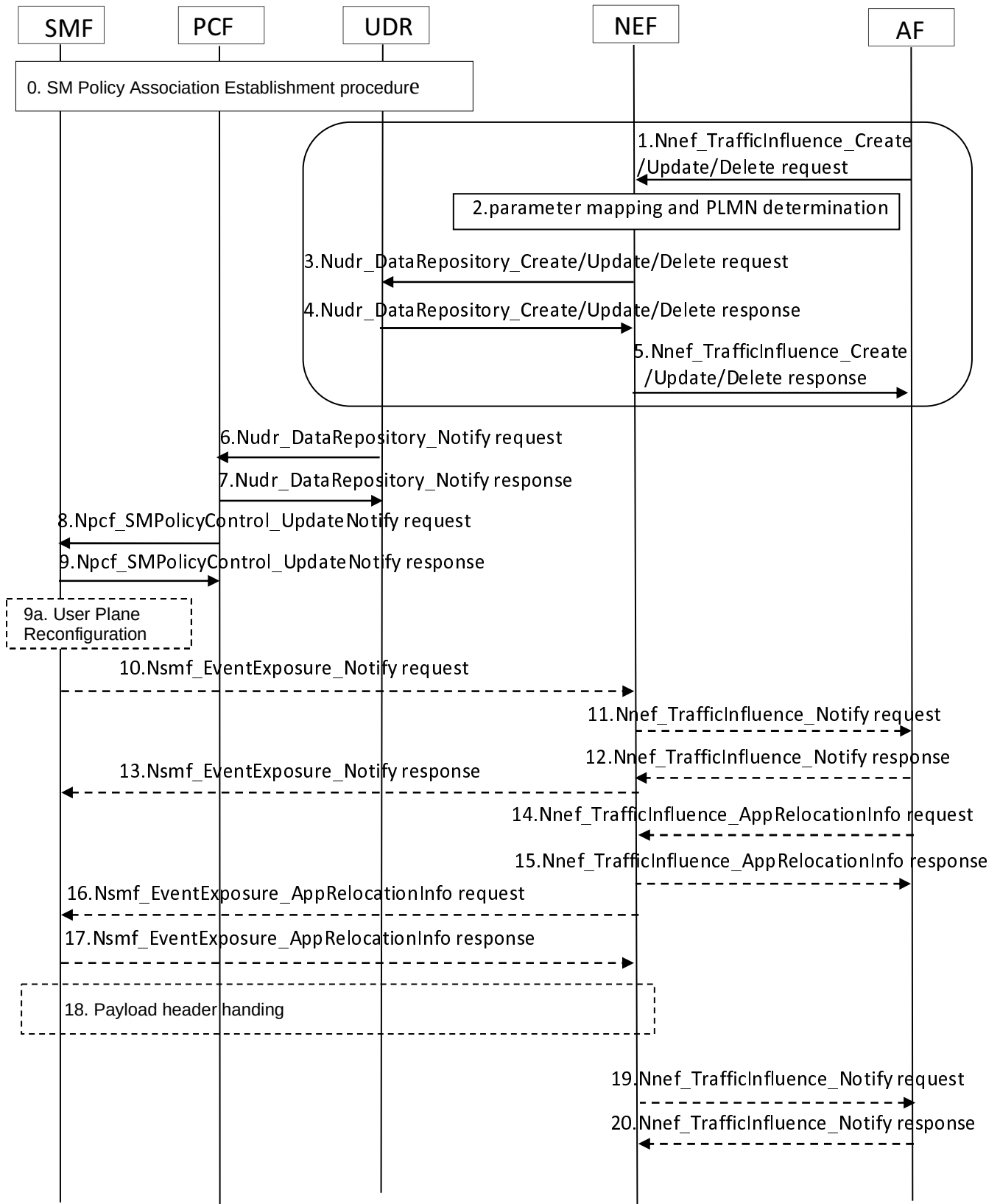
Figure 5.5.3.3-2: Processing AF requests to influence traffic routing for Sessions not identified by an UE address, affecting ongoing PDU session
