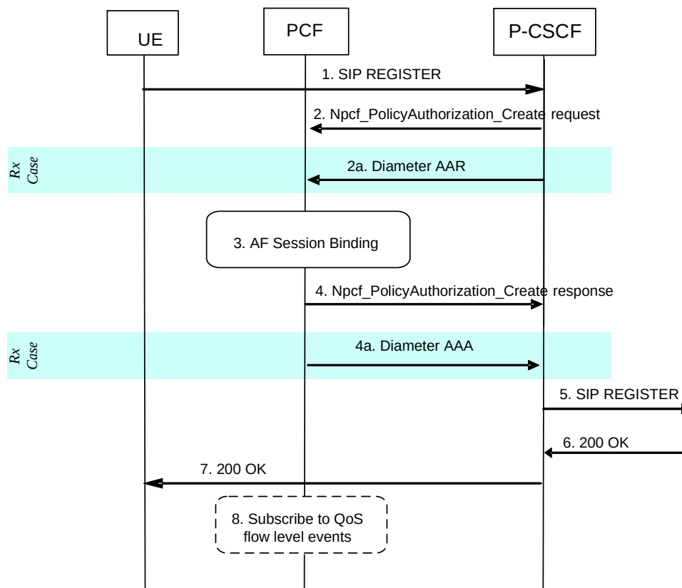
Figure B.7-1: Subscription to Notification of change of Access/IP-CAN Type at initial IMS Registration
