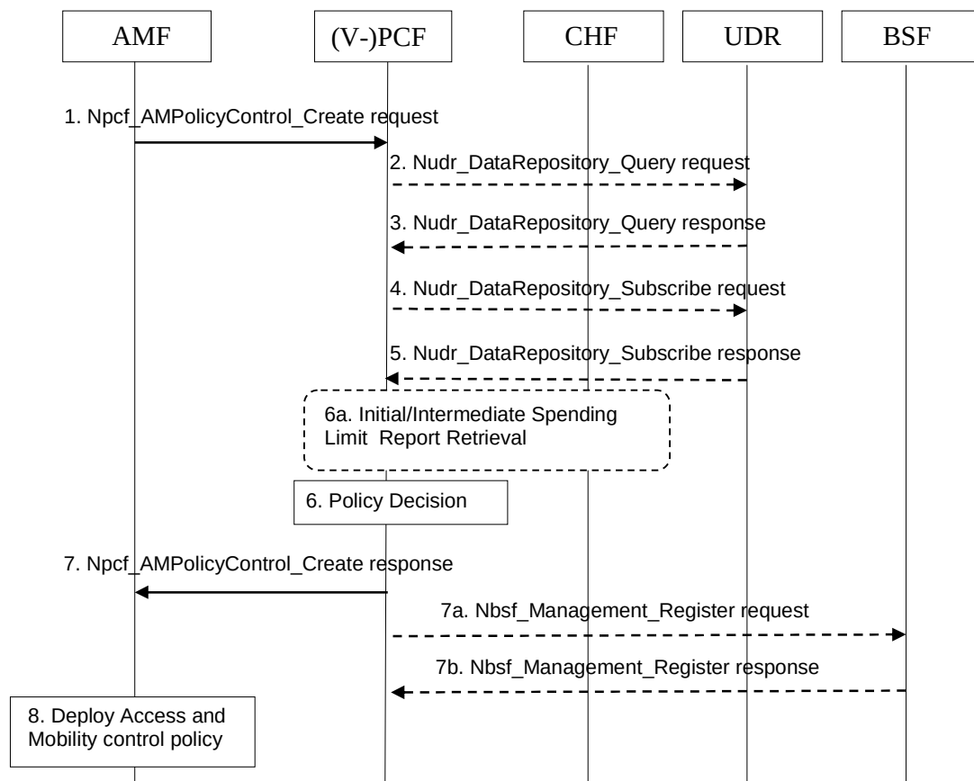
Figure 5.1.1-1: AM Policy Association Establishment procedure
