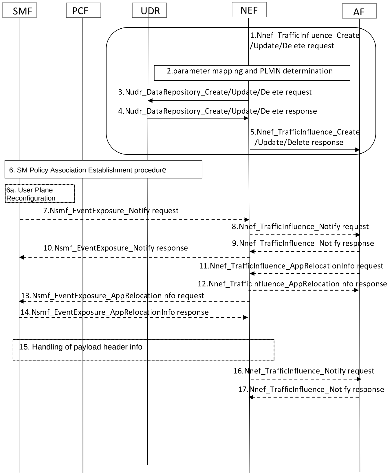
Figure 5.5.3.3-1: Processing AF requests to influence traffic routing for Sessions not identified by an UE address, affecting future PDU session
