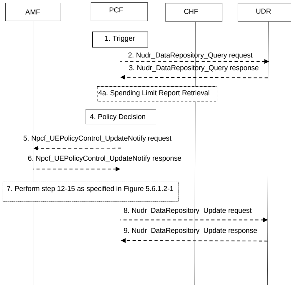
Figure 5.6.2.2.2-1: PCF-initiated UE Policy Association Modification procedure – Non-roaming
