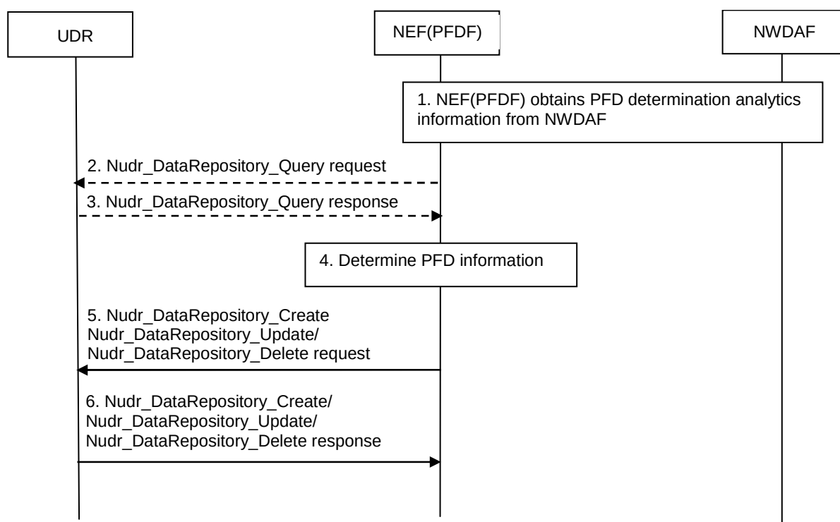
Figure 5.5.2.1A-1: PFD management based on NWDAF analytics
