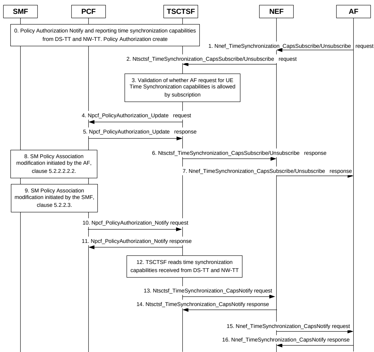
Figure 5.5.11.2-1: Exposure of UE availability and capabilities for Time Synchronization service
