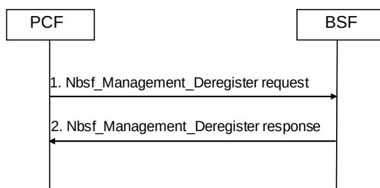
Figure 8.5.3-1: Binding information Deletion procedure
