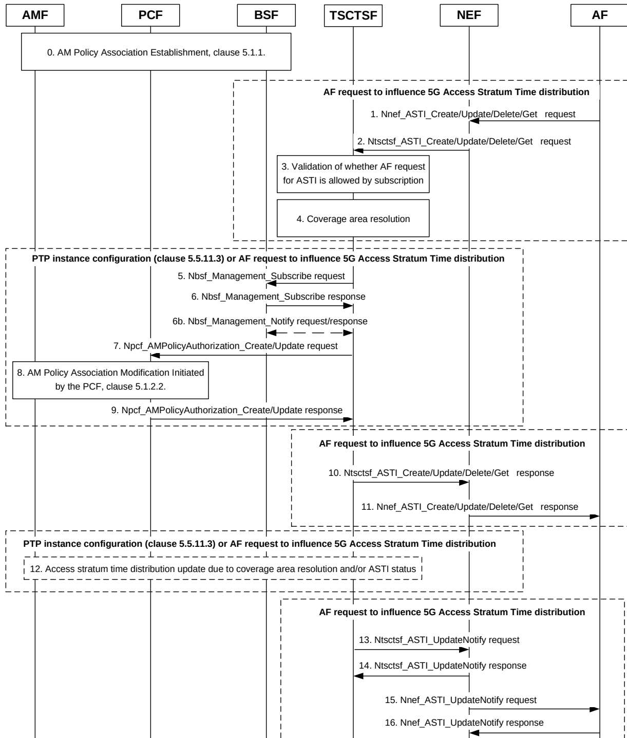
Figure 5.5.11.4-1: Management of 5G Access Stratum Time distribution
