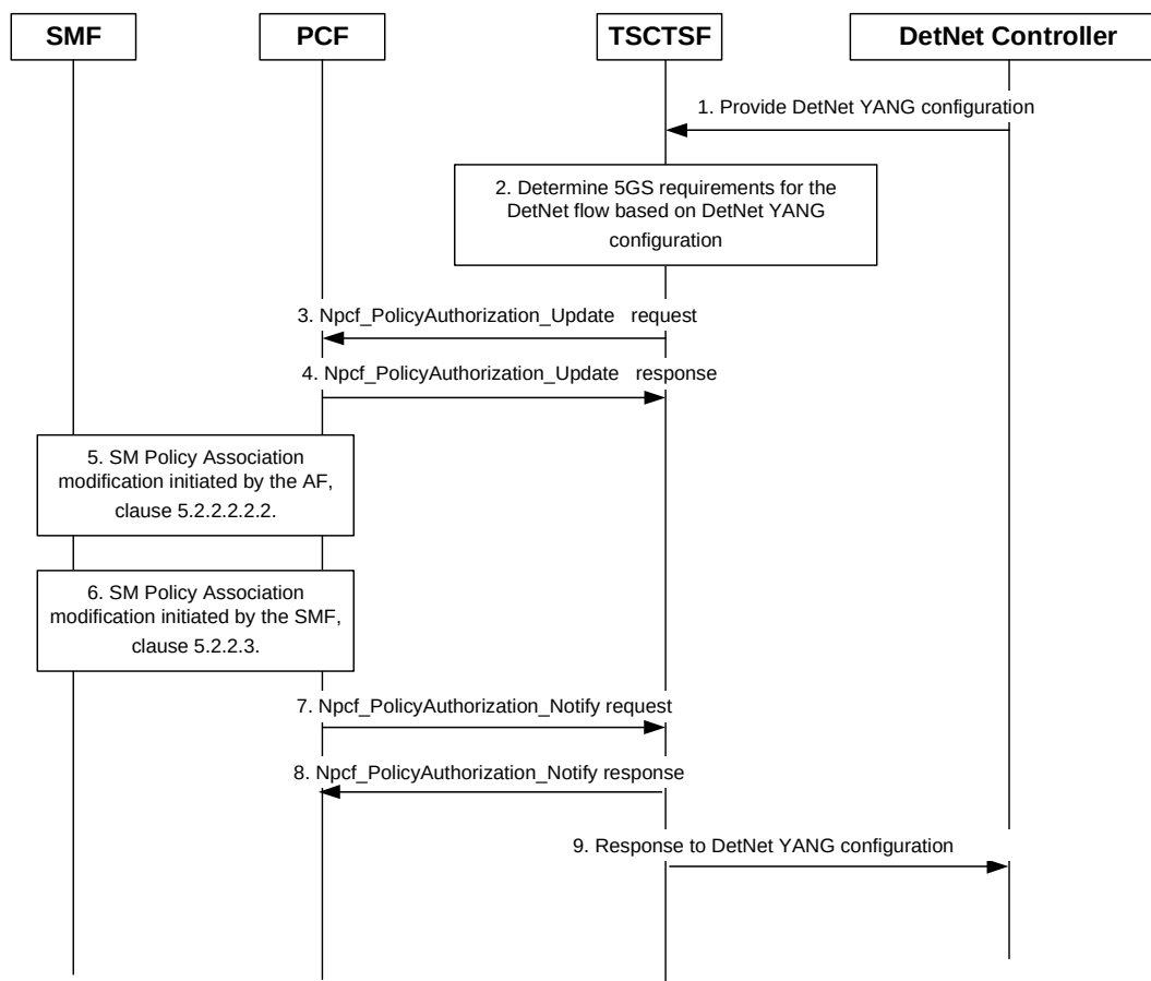
Figure 5.5.12.3-1: DetNet Node configuration
