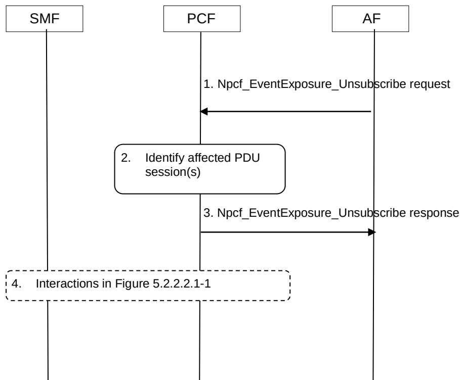
Figure 5.2.2.2.5-1: AF Request of application detection exposure termination triggers PCF-initiated SM Policy Association Modification procedure
