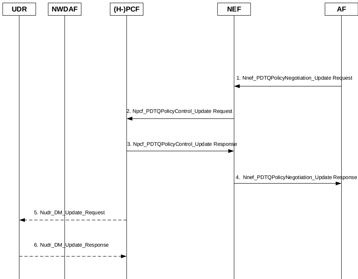
Figure 5.5.13A-1: Modification of PDTQ warning notification request indication procedure
