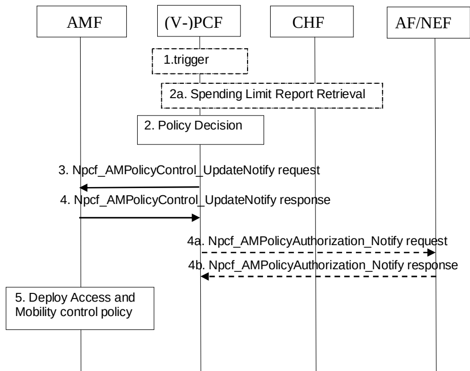
Figure 5.1.2.2-1: PCF-initiated AM Policy Association Modification procedure
