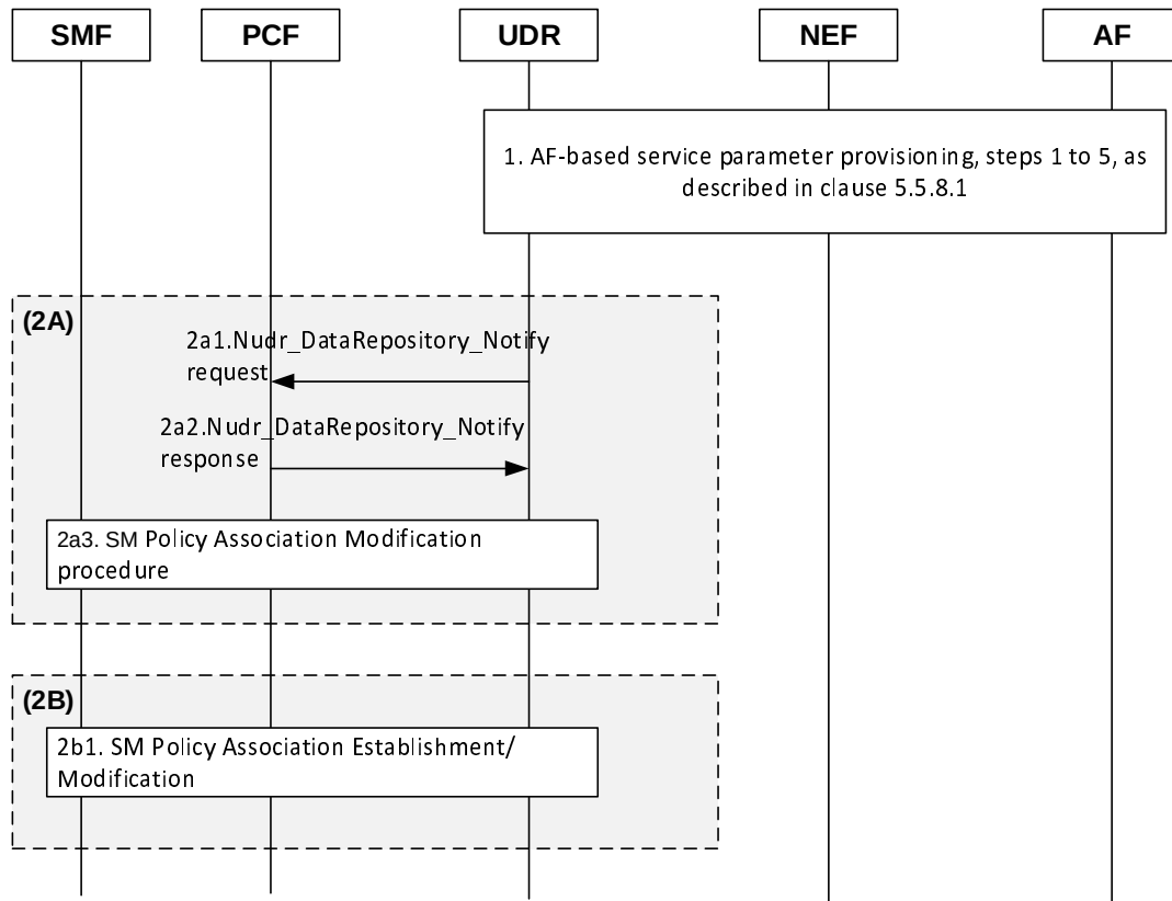
Figure 5.5.8.3-1: AF-based service parameter provisioning procedure of TNAP ID(s) to HPLMN of the UE
