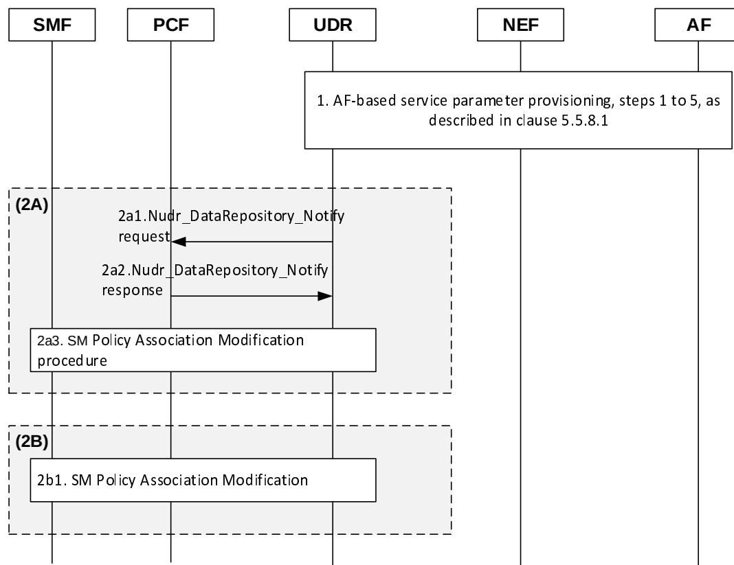
Figure 5.5.8.4-1: AF-based service parameter provisioning procedure of non-3GPP device identifier information to HPLMN of the UE
