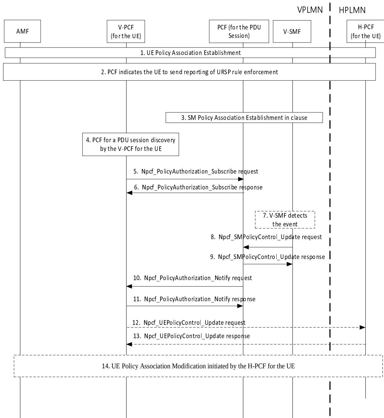
Figure 5.8.3-1: Forwarding of URSP Rule Enforcement Information (LBO roaming)
