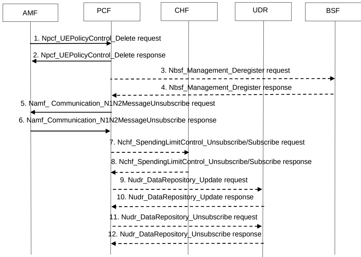
Figure 5.6.3.1.2-1: AMF-initiated UE Policy Association Termination procedure – Non-roaming
