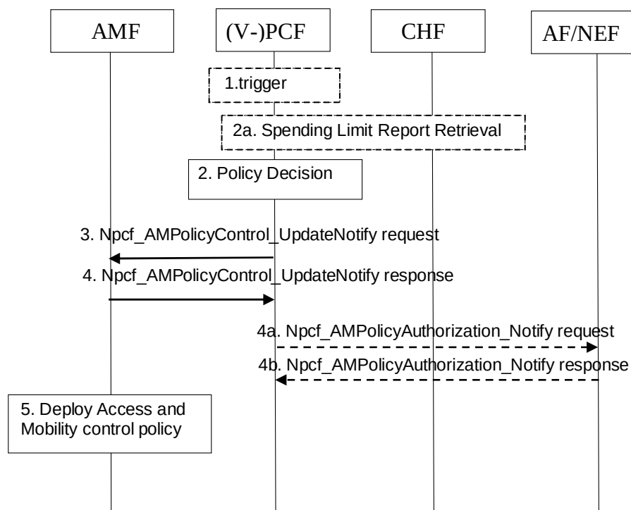
Figure 5.1.2.2-1: PCF-initiated AM Policy Association Modification procedure
