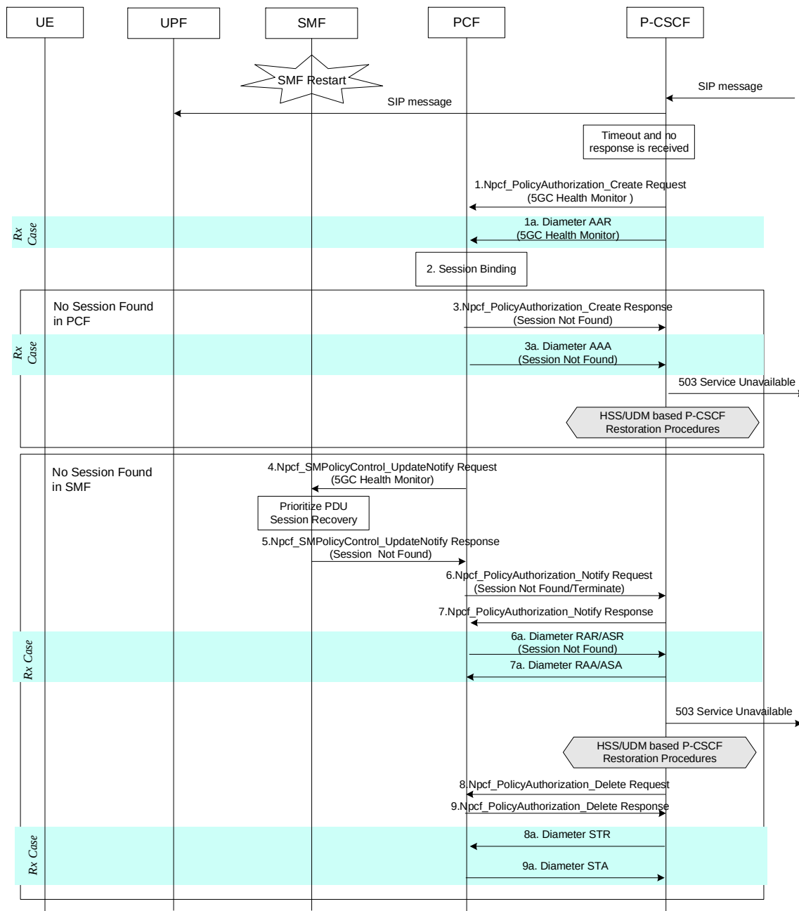
Figure B.15.2-1: P-CSCF initiated 5GC Network Functions Health Monitoring and SMF Failure
