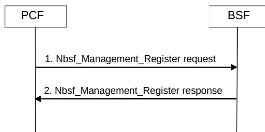
Figure 8.6.3.2-1: Binding information Creation procedure
