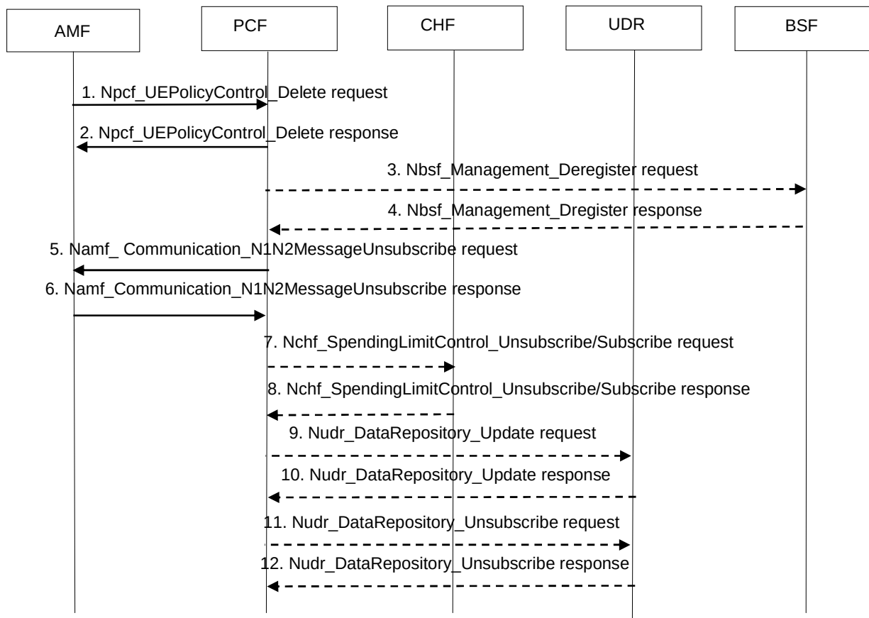
Figure 5.6.3.1.2-1: AMF-initiated UE Policy Association Termination procedure – Non-roaming
