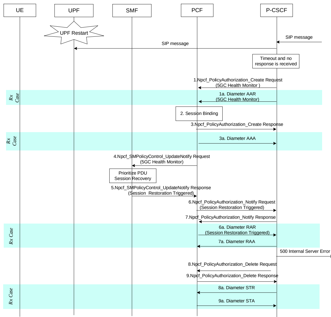
Figure B.15.1-1: P-CSCF initiated 5GC Network Functions Health Monitoring and UPF Failure
