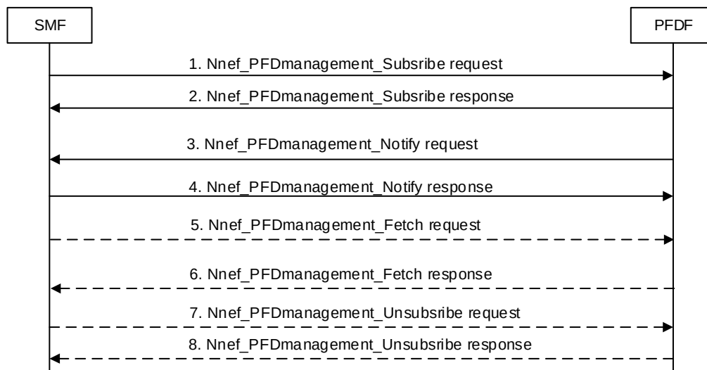
Figure 5.5.2.2-1: PFD management in the SMF
