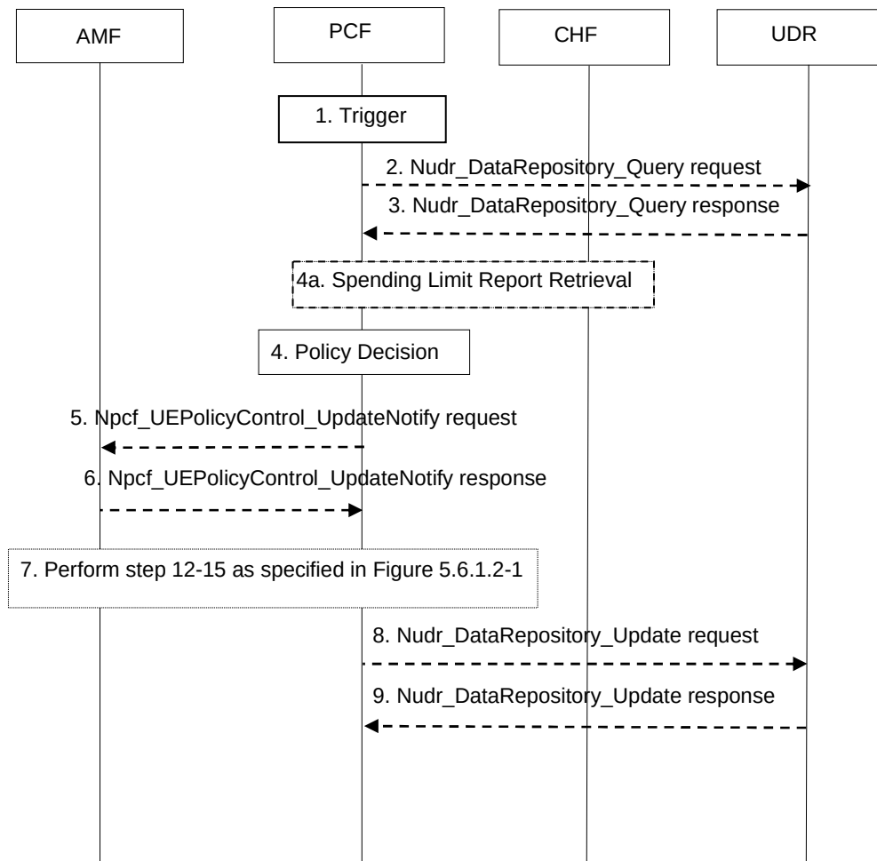
Figure 5.6.2.2.2-1: PCF-initiated UE Policy Association Modification procedure – Non-roaming
