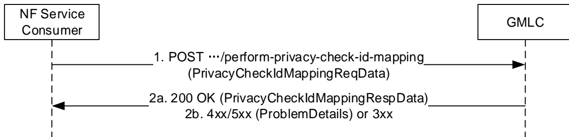
Figure 5.2.2.8.1-1: PrivacyCheckIdMapping Request/Response
