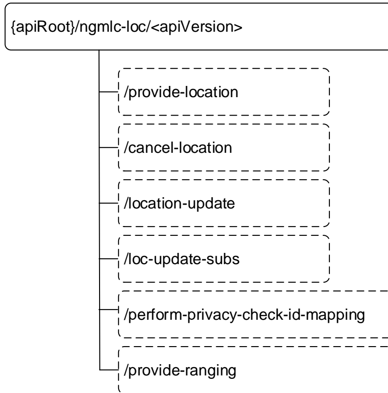
Figure 6.1.3.1-1: Custom operation URI structure of the Ngmlc_Location API
