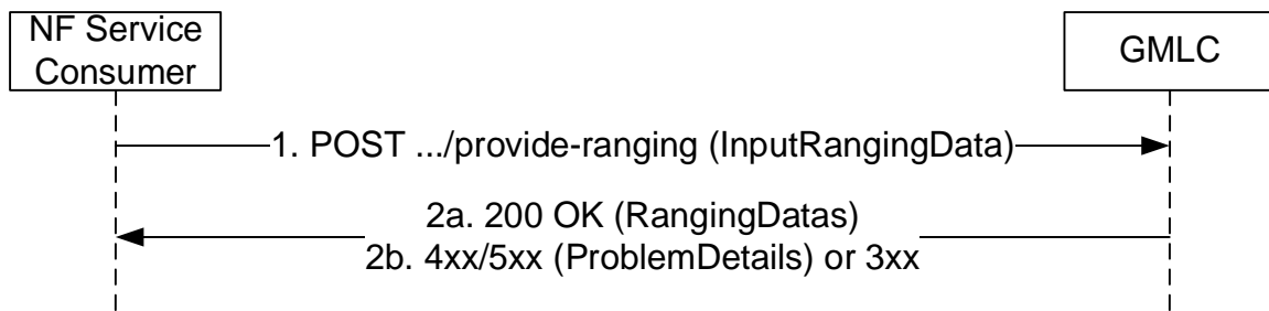
Figure 5.2.2.9.1: ProvideRanging Request/Response
