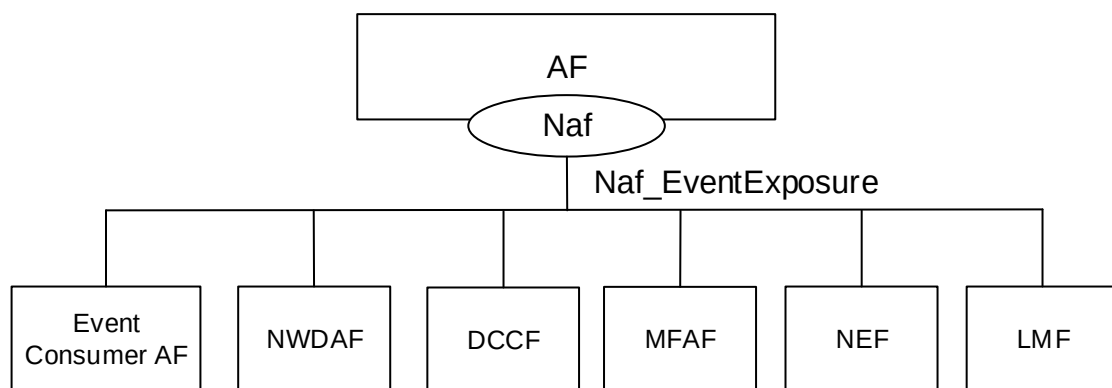
Figure 4.1.2-1: Naf_EventExposure service Architecture, SBI representation
