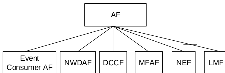
Figure 4.1.2-2: Naf_EventExposure service Architecture, reference point representation
