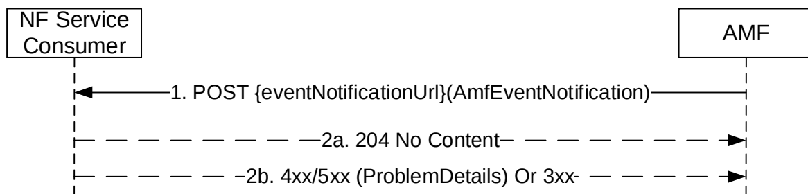
Figure 5.3.2.4.1-1 Notify
