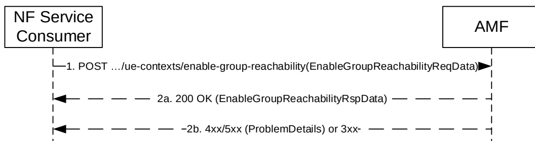
Figure 5.4.2.4.1-1: NF Service Consumer enabling the reachability of a list of UEs
