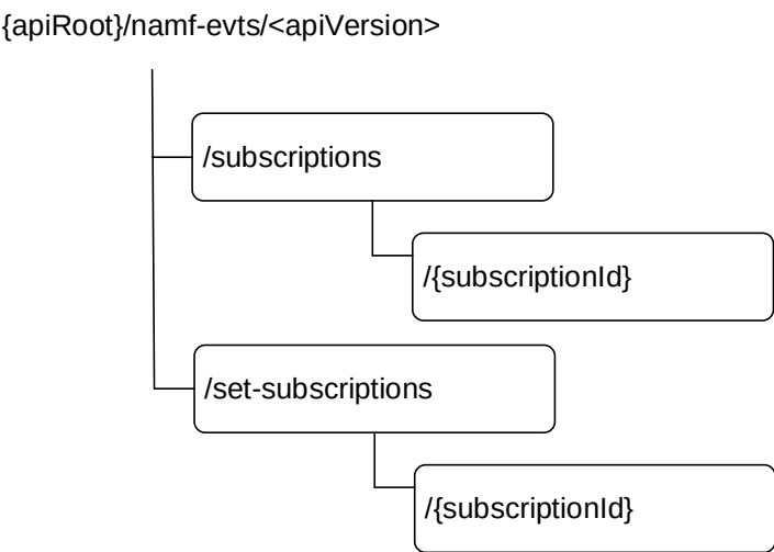
Figure 6.2.3.1-1: Resource URI structure of the Namf_EventExposure API
