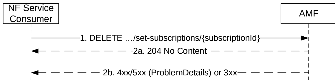
Figure 5.3.2.2.2-2 Unsubscribe for an AMF Set level Bulk Subscription
