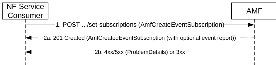
Figure 5.3.2.2.2 Subscribe service operation for an AMF Set level Bulk Subscription
