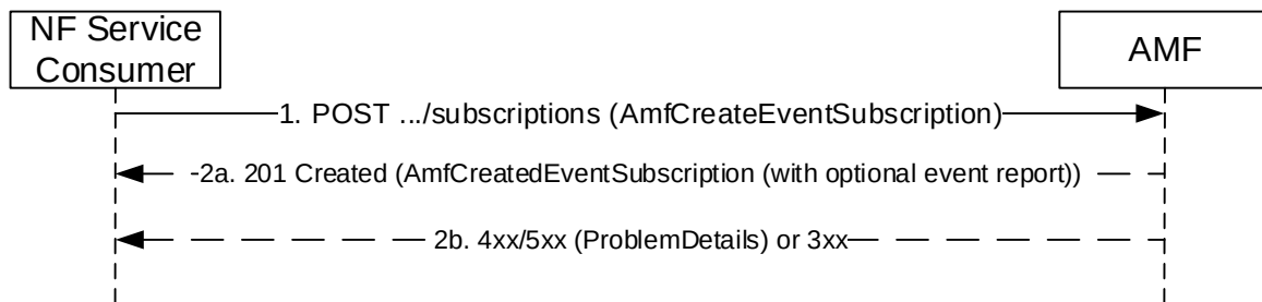
Figure 5.3.2.2.1 Subscribe service operation
