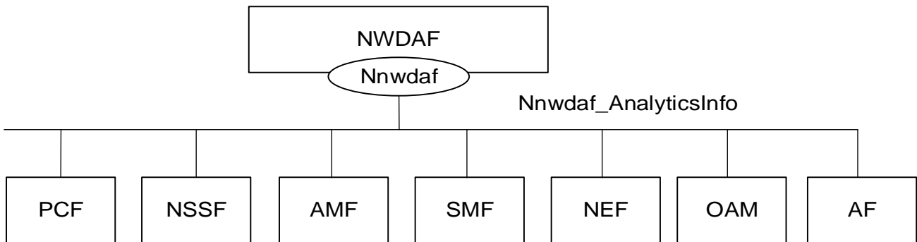
Figure 4.3.1.2-1: Reference Architecture for the Nnwdaq_AnalyticsInfo Service; SBI representation
