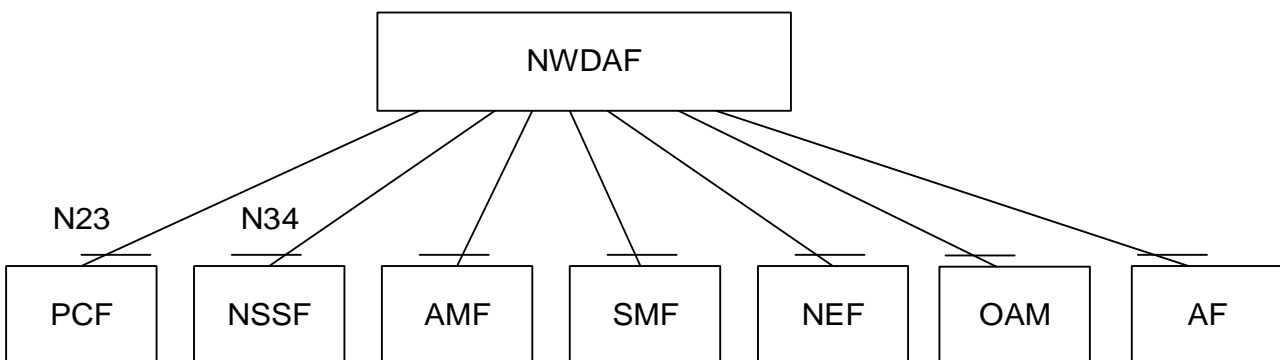
Figure 4.3.1.2-2: Reference Architecture for the Nnwdaq_AnalyticsInfo Service: reference point representation
