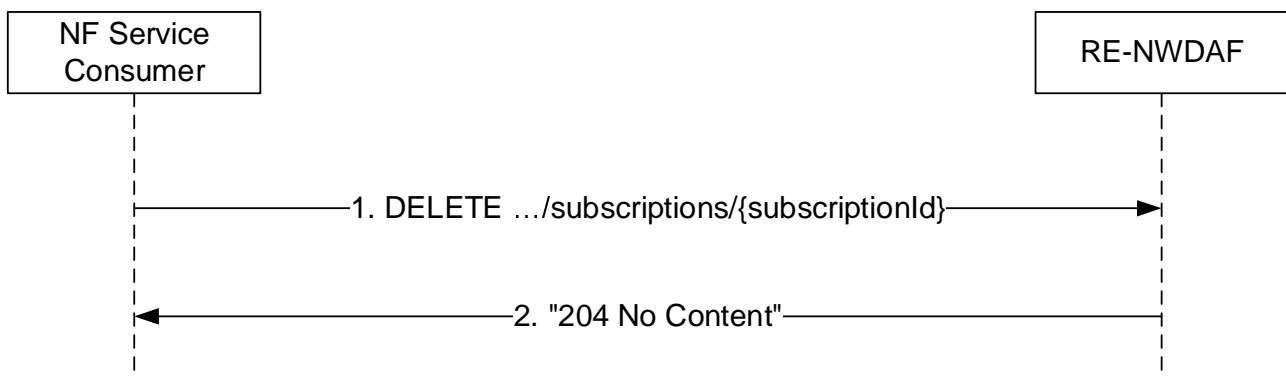
Figure 4.8.2.3.2-1: NF service consumer unsubscribes from notifications
