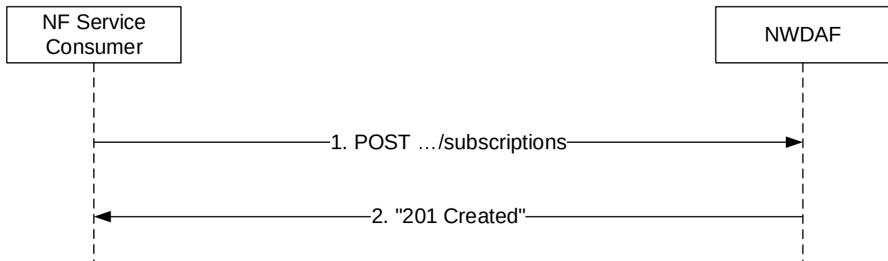
Figure 4.7.2.4.2-1: NF service consumer subscribes to notifications
