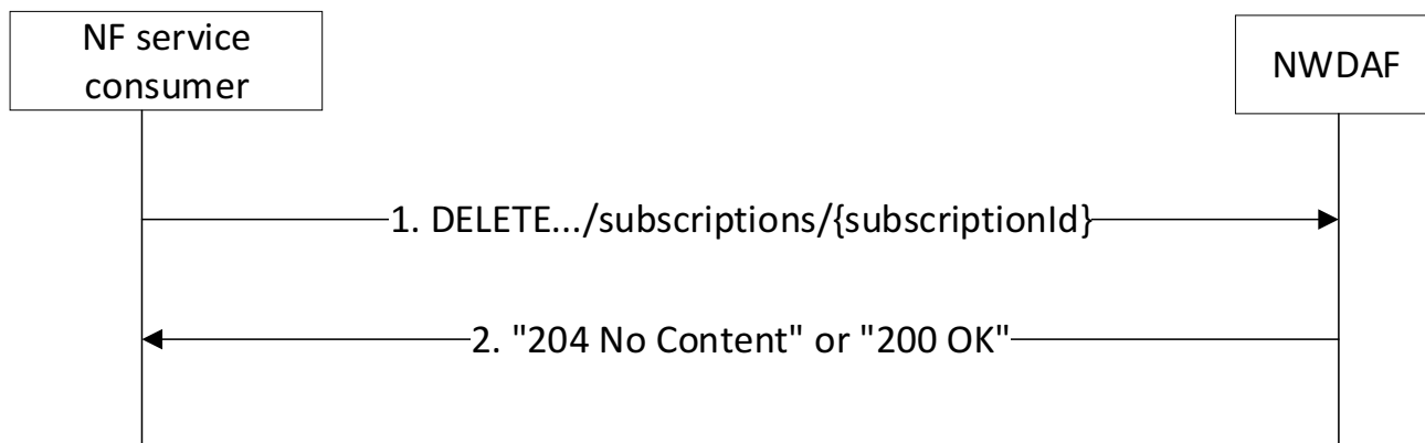
Figure 4.4.2.3.2-1: NF service consumer unsubscribes from data notifications
