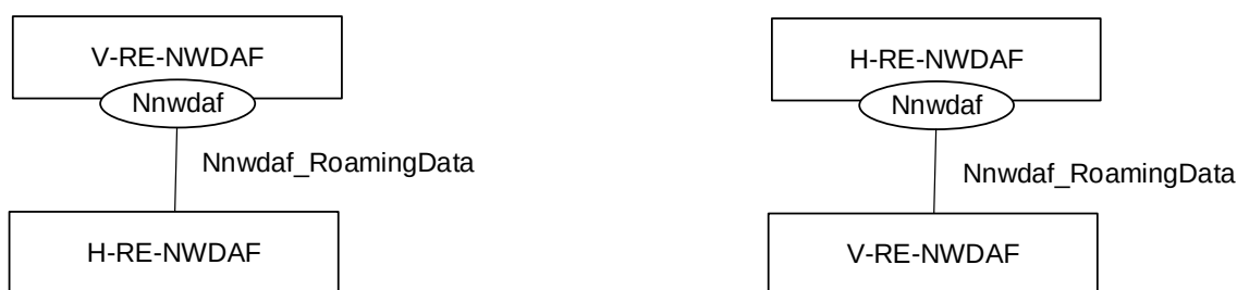
Figure 4.8.1.2-1: Reference Architecture for the Nnwdaf_RoamingData Service; SBI representation
