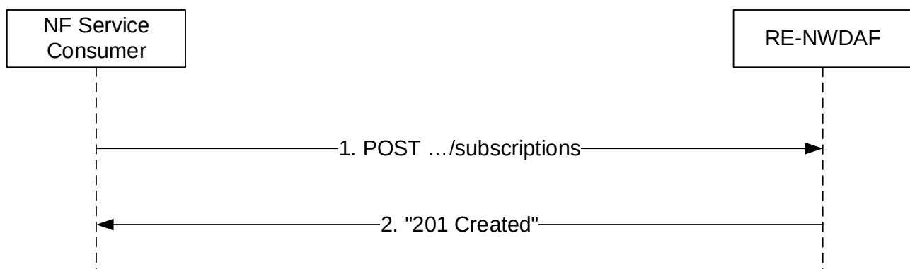
Figure 4.8.2.2.2-1: NF service consumer subscribes to notifications
