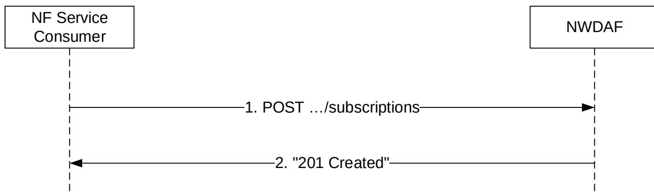
Figure 4.10.2.2.2-1: NF service consumer subscribes to VFL training information
