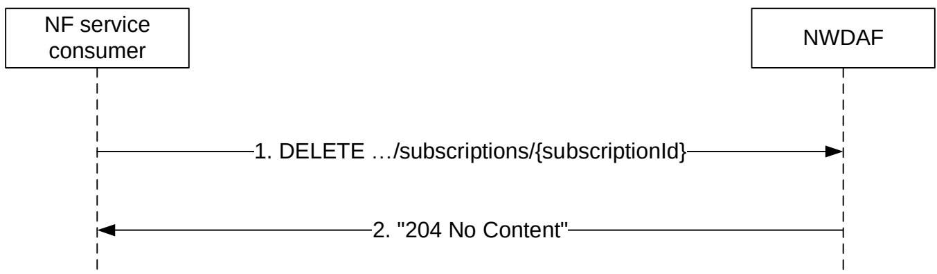
Figure 4.11.2.3.2-1: NF service consumer unsubscribes from VFL inference notifications
