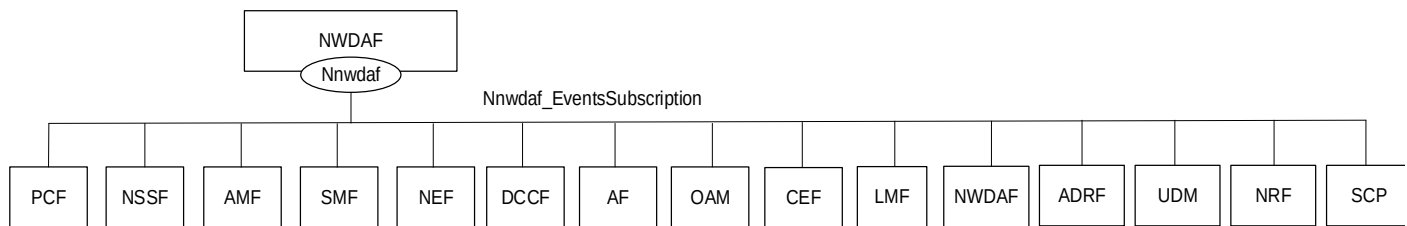
Figure 4.2.1.2-1: Reference Architecture for the Nnwdaf_EventsSubscription Service; SBI representation
