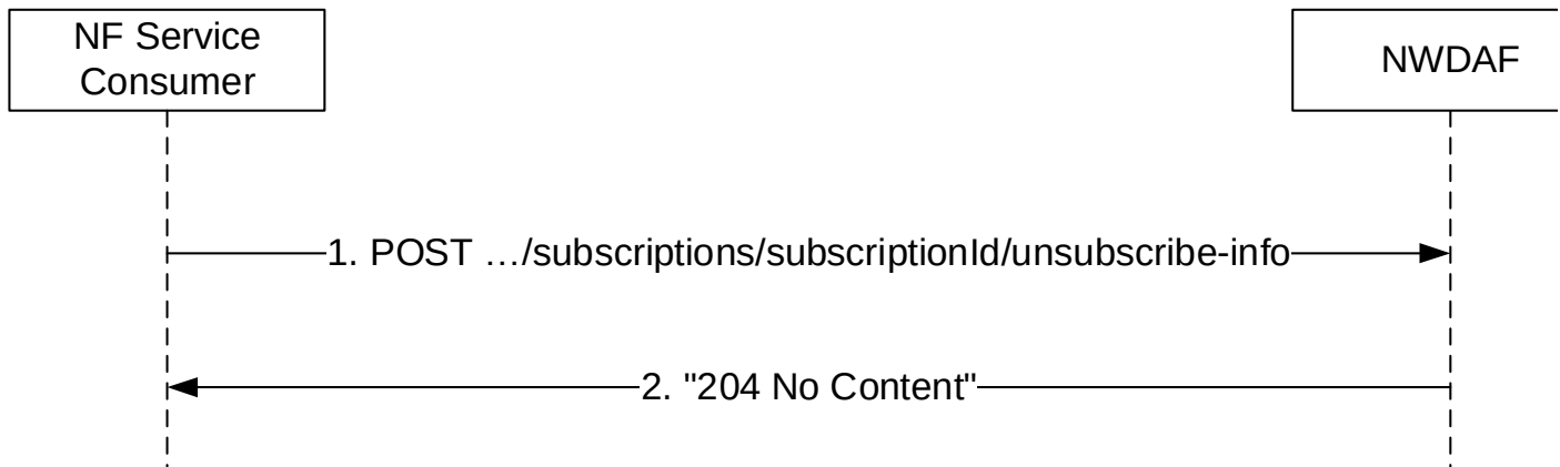
Figure 4.6.2.3.3-1: NF service consumer unsubscribes from notifications providing additional information
