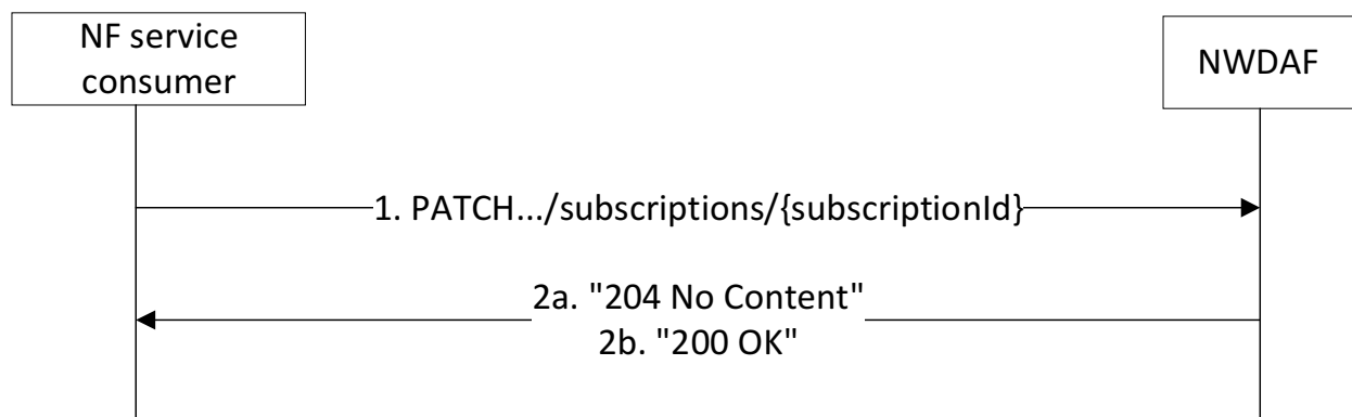
Figure 4.11.2.2.4-1: Partial modification of VFL inference subscription information using HTTP PATCH
