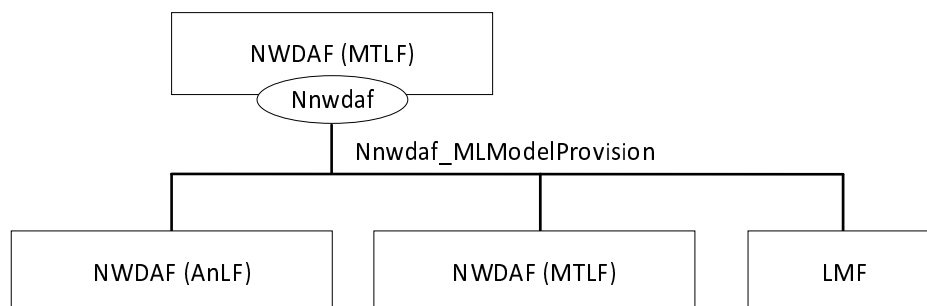
Figure 4.5.1.2-1: Reference Architecture for the Nnwdaf_MLModelProvision Service; SBI representation
