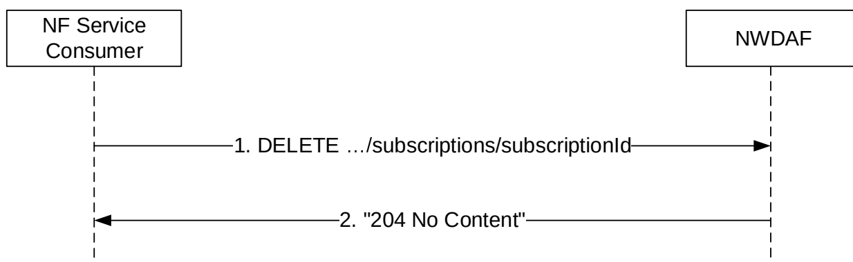
Figure 4.7.2.5.2-1: NF service consumer unsubscribes from notifications
