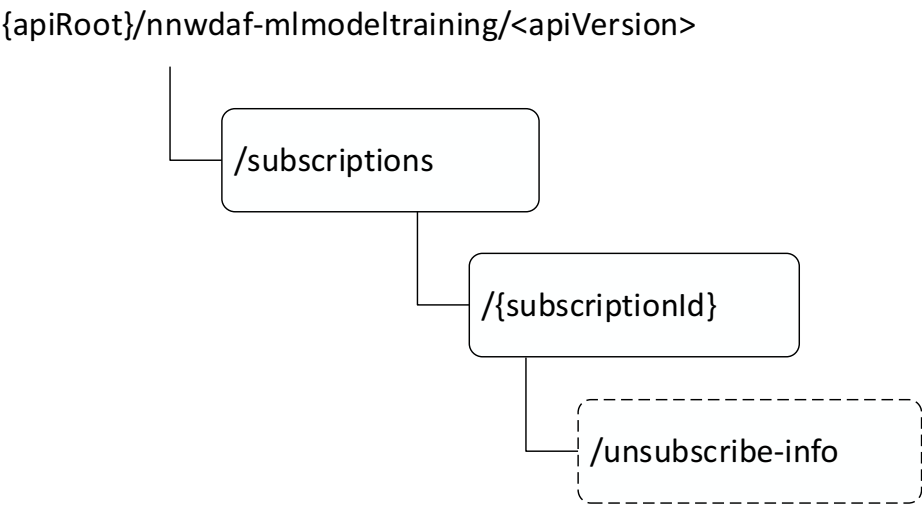
Figure 5.5.3.1-1: Resource URI structure of the Nnwdaf_MLModelTraining API
