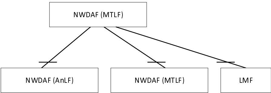
Figure 4.5.1.2-2: Reference Architecture for the Nnwdaf_MLModelProvision Service: reference point representation
