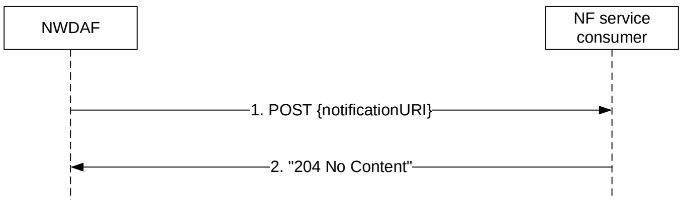
Figure 4.11.2.4.2-1: NWDAF notifies the subscribed VFL inference event
