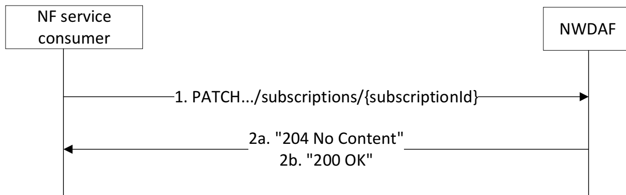
Figure 4.10.2.2.4-1: Partial modification of Individual VFL Training Subscription using HTTP PATCH
