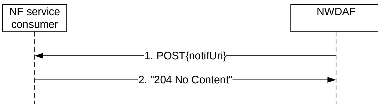
Figure 4.10.2.4.2-1: NWDAF notifies the subscribed event
