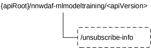
Figure 5.5.4.1-1: Custom operation URI structure of the Nnwdaf_MLModelTraining API
