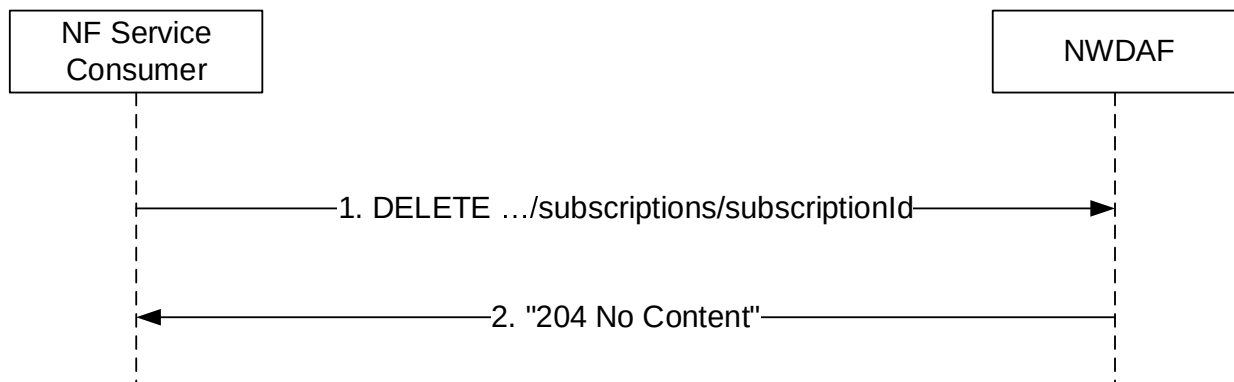
Figure 4.10.2.3.2-1: NF service consumer unsubscribes from VFL training information
