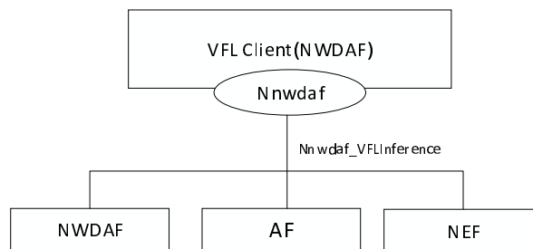
Figure 4.11.1.2-1: Reference Architecture for the Nnwdaf_VFLInference service; SBI representation
