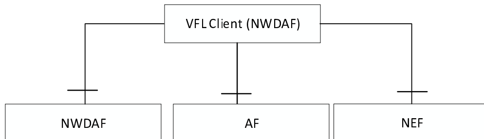
Figure 4.11.1.2-2: Reference Architecture for the Nnwdaf_VFLInference service: reference point representation
