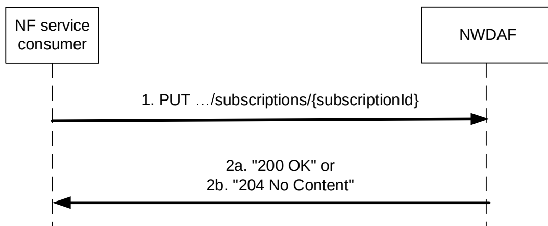
Figure 4.10.2.2.3-1: NF service consumer updates subscription to VFL training information
