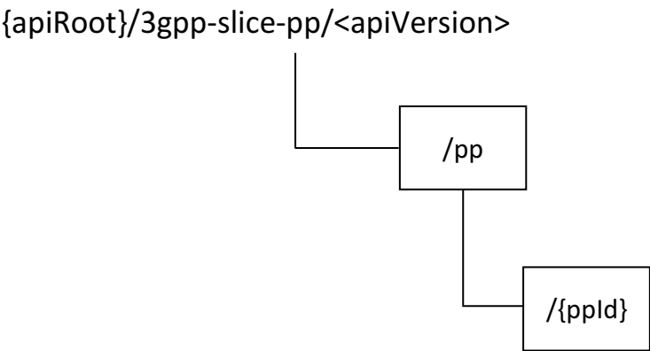
Figure 5.34.2.1-1: Resource URI structure of the SliceParamProvision API
