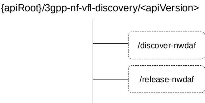
Figure 5.48.3.1-1: Custom operation URI structure of the VFLNFDISCOVERY API
