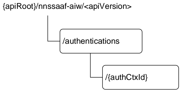
Figure 6.2.3.1-1: Resource URI structure of the AIW API
