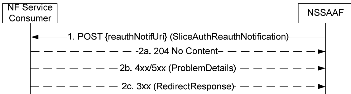
Figure 5.2.2.3.1-1: Re-authentication Notification
