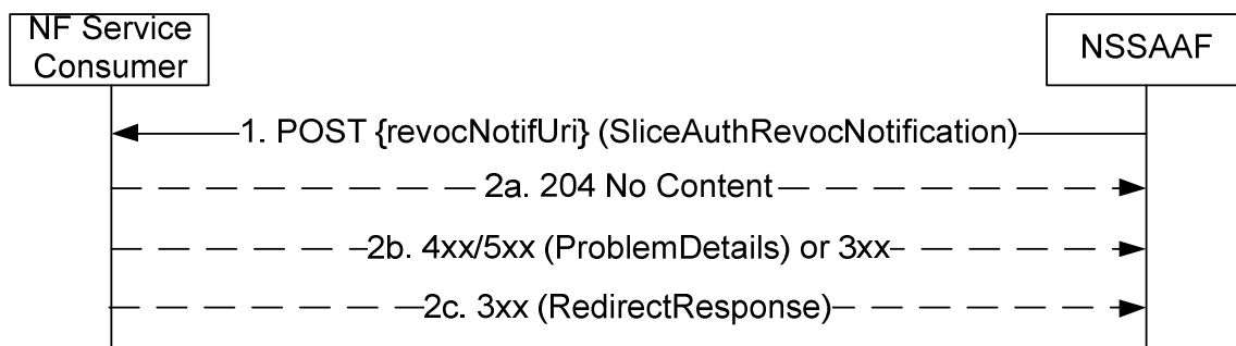
Figure 5.2.2.4.1-1: Revocation Notification
