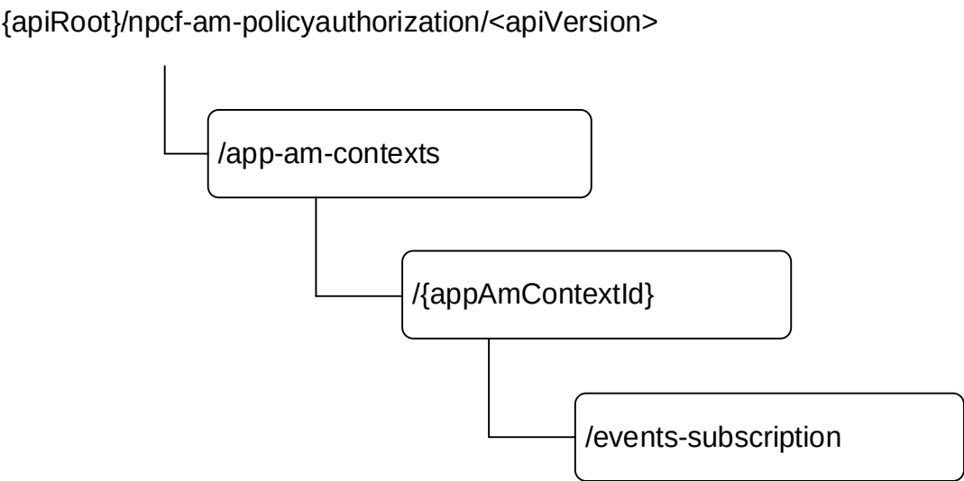
Figure 5.3.1-1: Resource URI structure of the Npcf_AMPolicyAuthorization API
