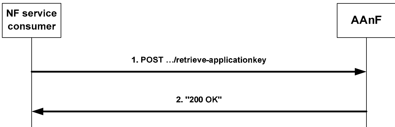
Figure 4.2.2.3.2-1: NF service consumer retrieve AKMA Application Key information
