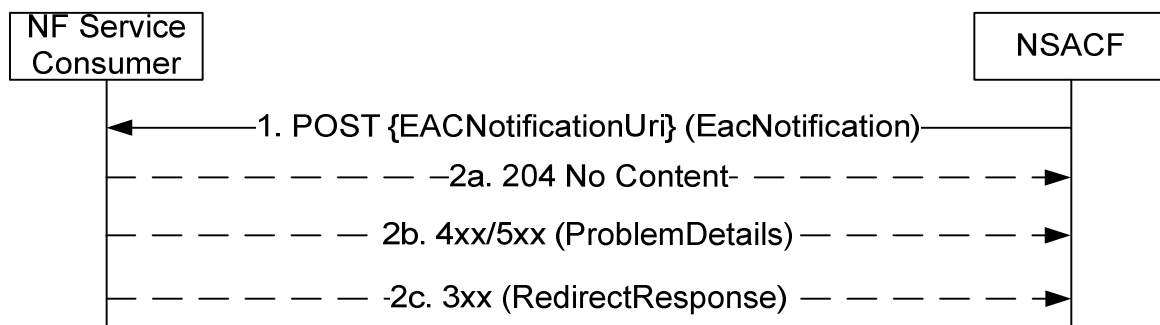
Figure 5.2.2.2.3-1: NSACF initiated EAC mode configuration procedure
