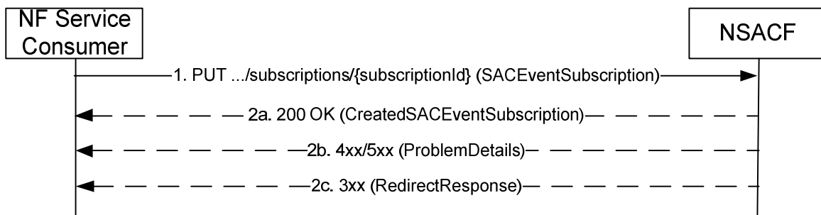
Figure 5.3.2.2.3-2 Subscription Complete Replacement
