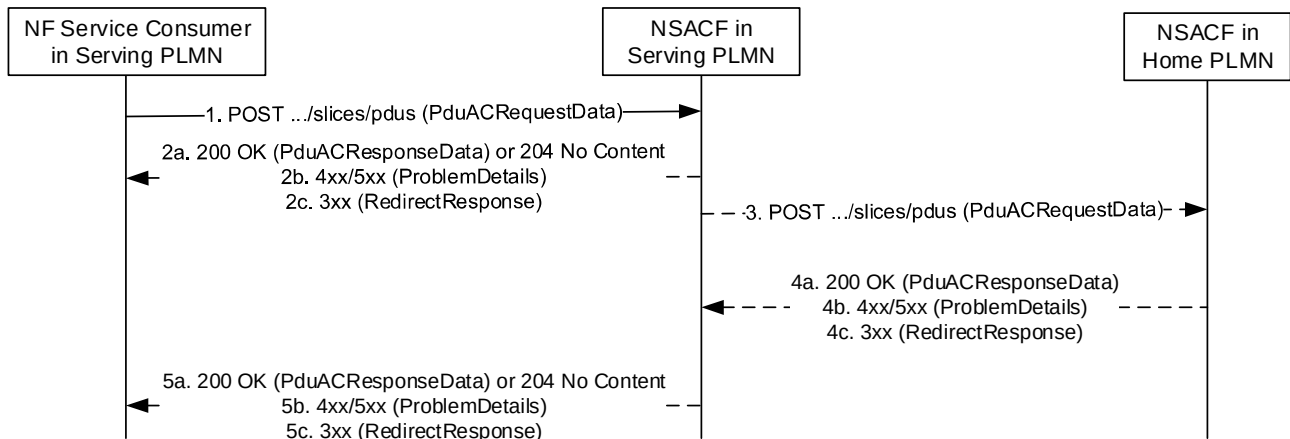
Figure 5.2.2.4.5-1: HPLMN Delegated NSAC procedure for controlling the number of LBO PDU sessions
