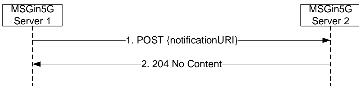
Figure 5.4.2.4.2-1:MSGin5G Server Notification about Messaging Topic List
