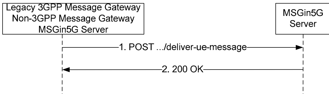
Figure 5.3.2.4.2-1: Legacy 3GPP UE or Non-3GPP UE Originating MSGin5G Message Delivery
