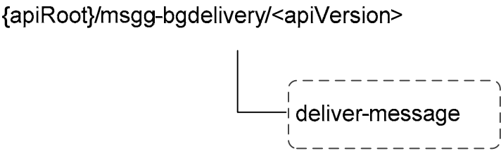
Figure 9.3.3.1-1: Custom operation URI structure of the MSGG_BGDelivery API
