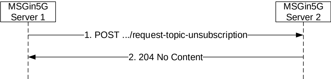
Figure 5.4.2.6.2-1:Unsubscribing to Messaging Topic(s)
