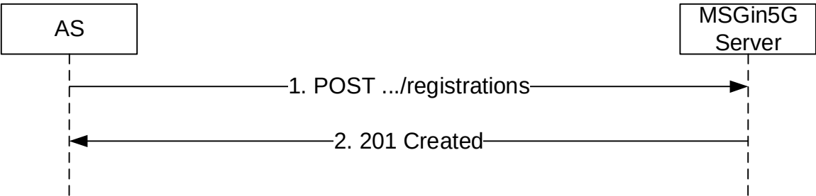
Figure 5.2.2.2.2-1: AS Registering to MSGin5G Server
