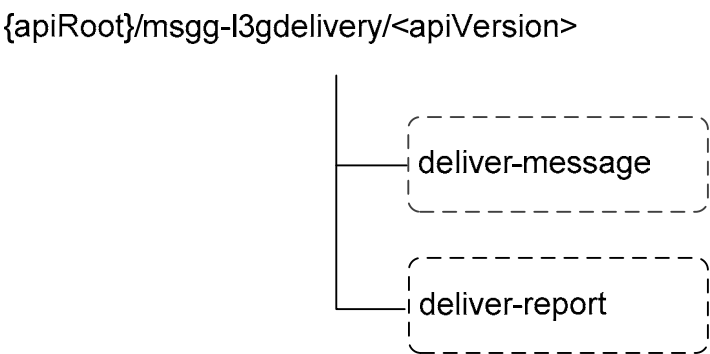
Figure 9.1.3.1-1: Custom operation URI structure of the MSGG_L3GDelivery API
