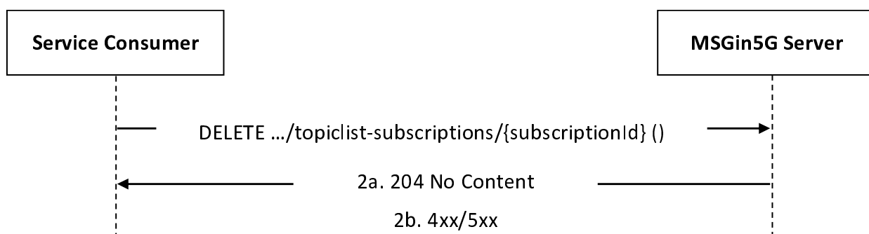
Figure 5.4.2.3.2-1: MSGin5G Server Unsubscribing to Messaging Topic List
