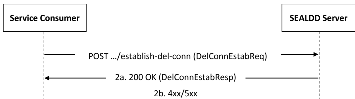
Figure 5.3.2.6.2-1: Procedure for SEALDD Data Storage Delivery Connection Establishment Request
