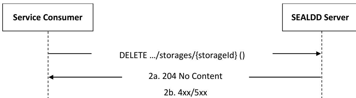
Figure 5.3.2.3.3-1: Procedure for Data Storage Deletion
