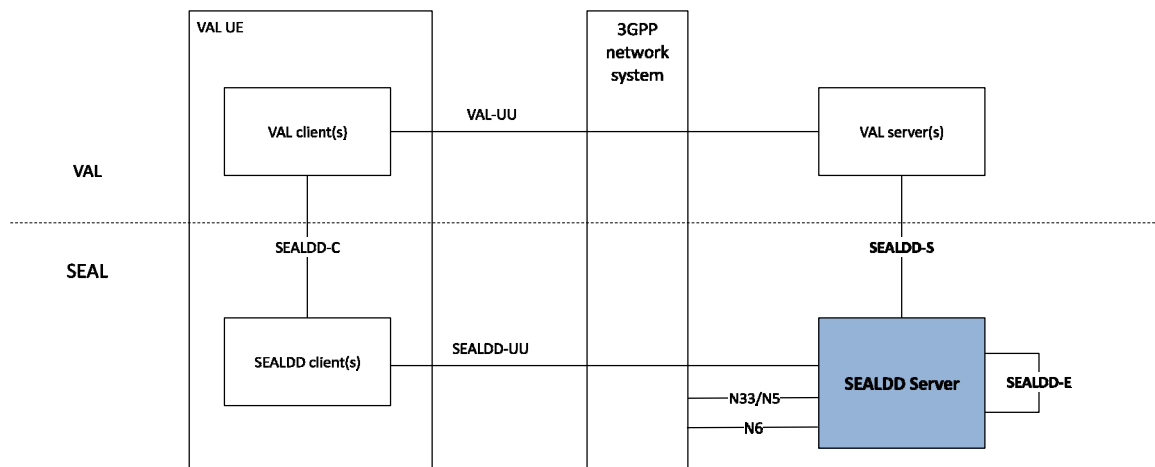
Figure 4-1: SEALDD Enabler Layer functional model
