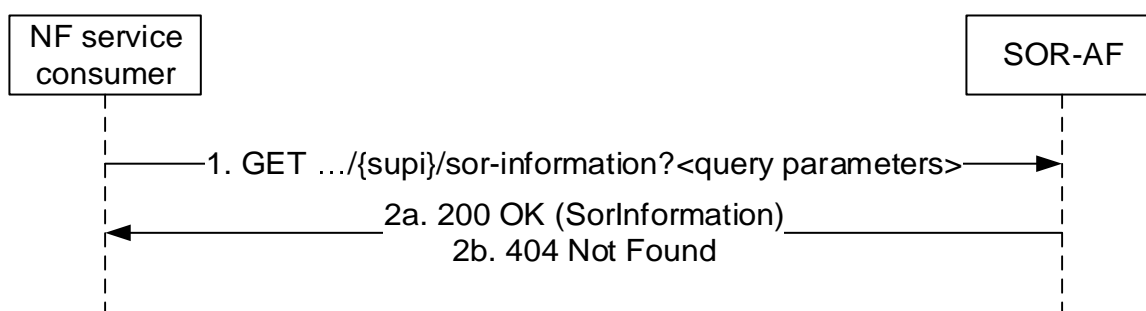
Figure 5.2.2.2.2-1: SoR Information Retrieval Procedure
