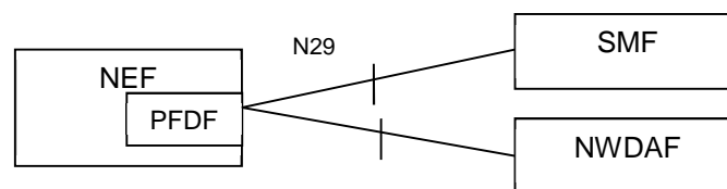
Figure 4.1.2-2: Reference Architecture for the Nnef_PFDmanagement Service; reference point representation
