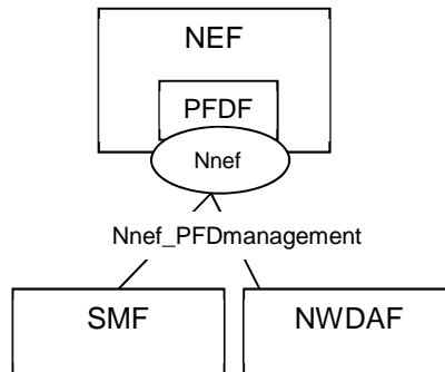
Figure 4.1.2-1: Reference Architecture for the Nnef_PFDmanagement Service; SBI representation
