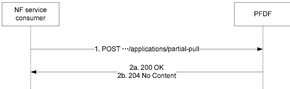
Figure 4.2.2.3-1: Retrieval of PFDs by the partial pull
