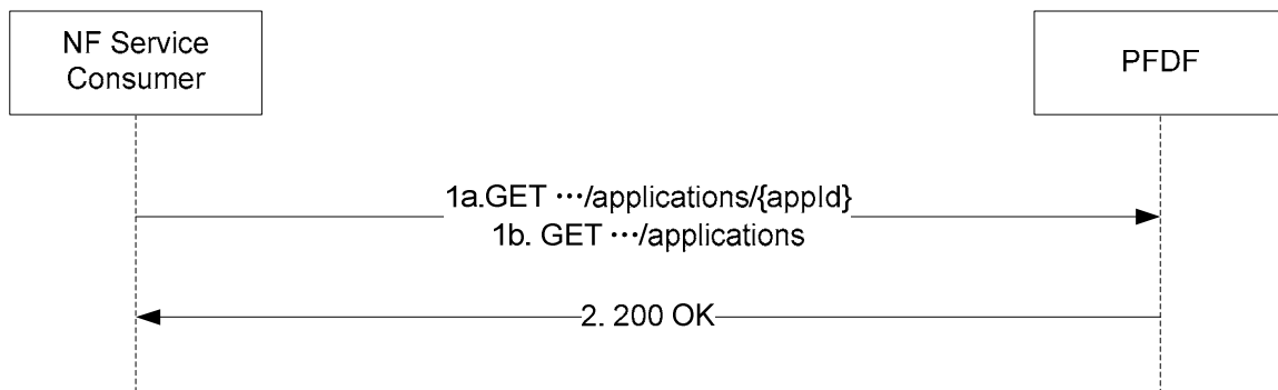
Figure 4.2.2.2-1: Retrieval of PFDs by the full pull
