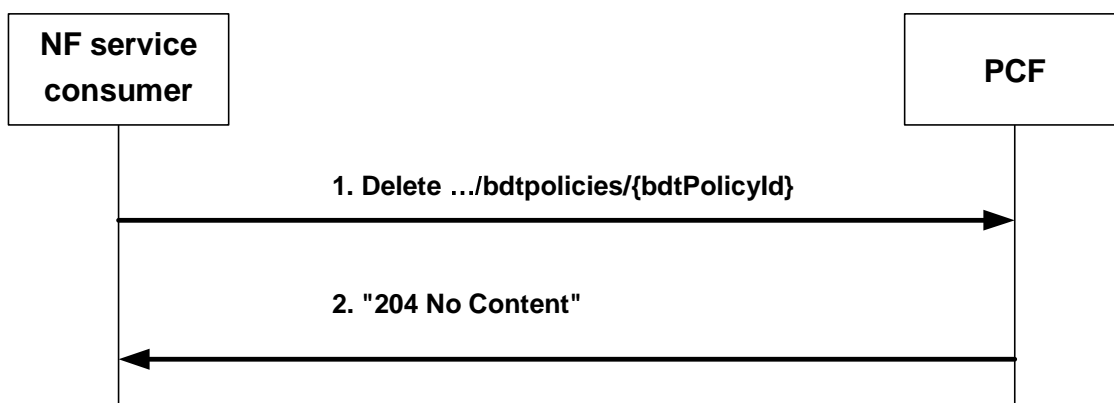
Figure 4.2.5.2-1 Deletion of BDT policy.
