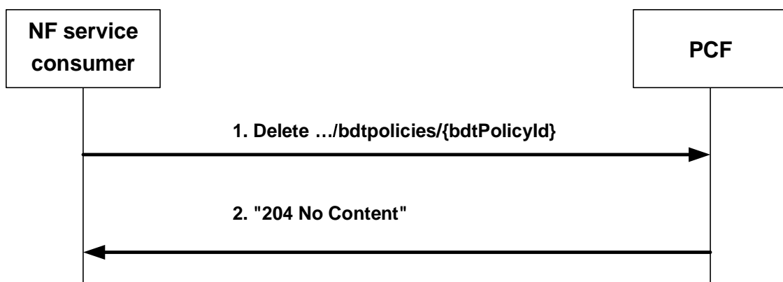
Figure 4.2.5.2-1 Deletion of BDT policy.
