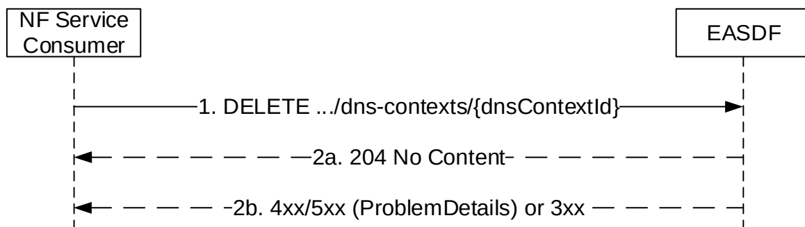
Figure 5.2.2.4.1-1: DNS context deletion
