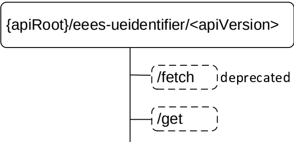
Figure 8.3.3.1-1: Custom operation URI structure of the Eees_UEIdentifier API
