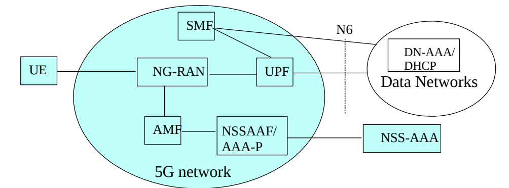
Figure 6-1: Reference Architecture for 5G Network Interworking
