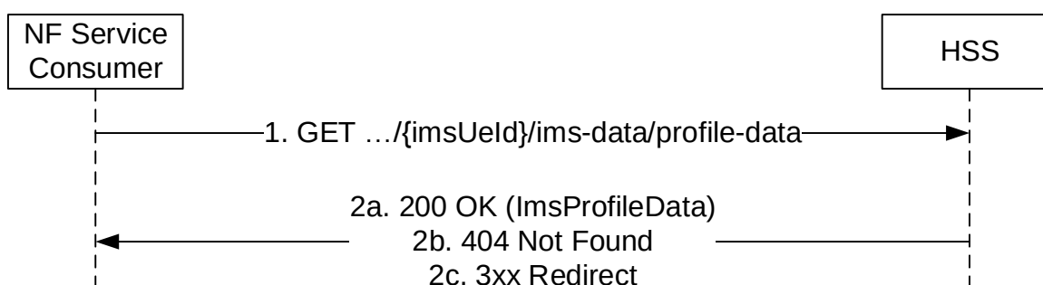
Figure 5.3.2.2.4.1-1: IMS User Profile Retrieval
