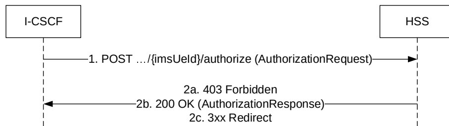
Figure 5.2.2.5.2-1: Authorization
