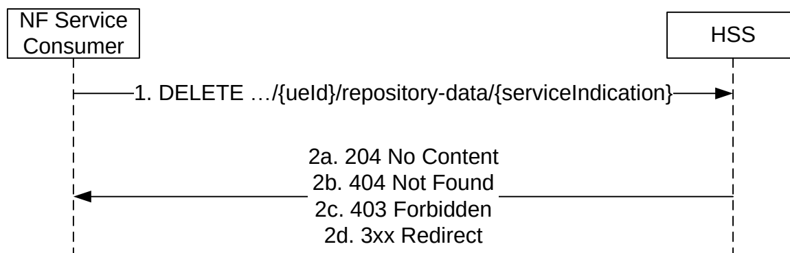
Figure 5.3.2.7.3-1: Deleting repository data
