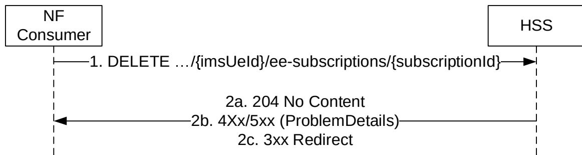
Figure 5.7.2.3.2-1: Deletion of a subscription to a specific subscriber related IMS event
