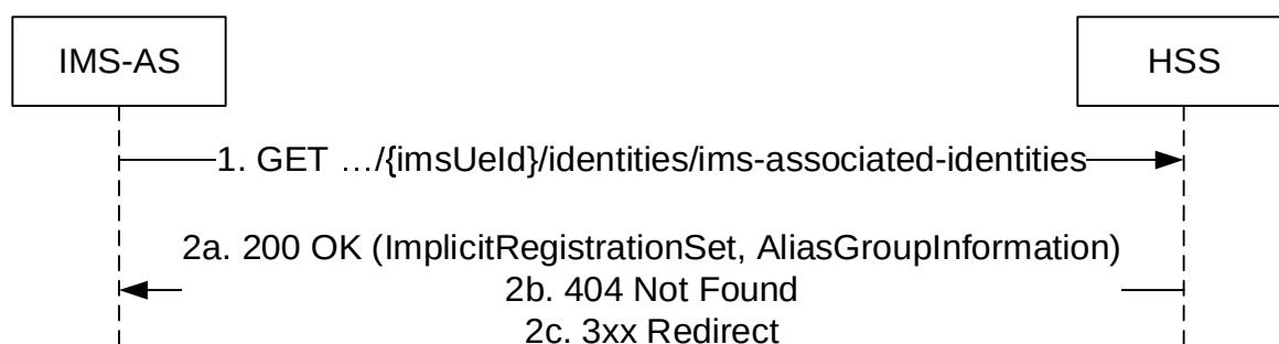
Figure 5.3.2.2.1-1: IMS Identity Data Retrieval
