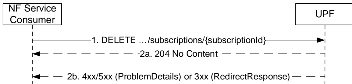
Figure 5.2.2.2A.1-1 Unsubscribing from UPF events
