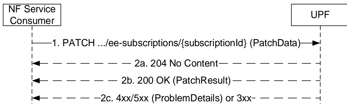
Figure 5.2.2.3-1: Modification of a subscription
