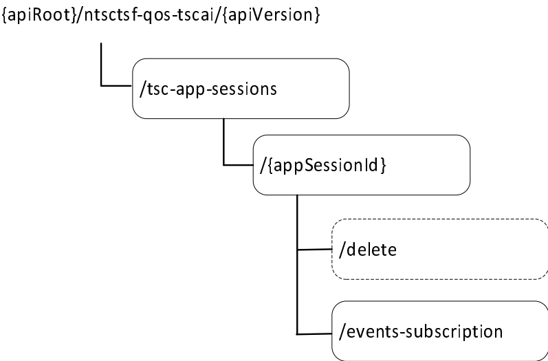
Figure 6.2.3.1-1: Resource URI structure of the Ntsctsf_QoSandTSCAssistance API
