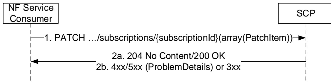
Figure 5.2.2.2.3-1: Modification of subscription for SCP Event Exposure
