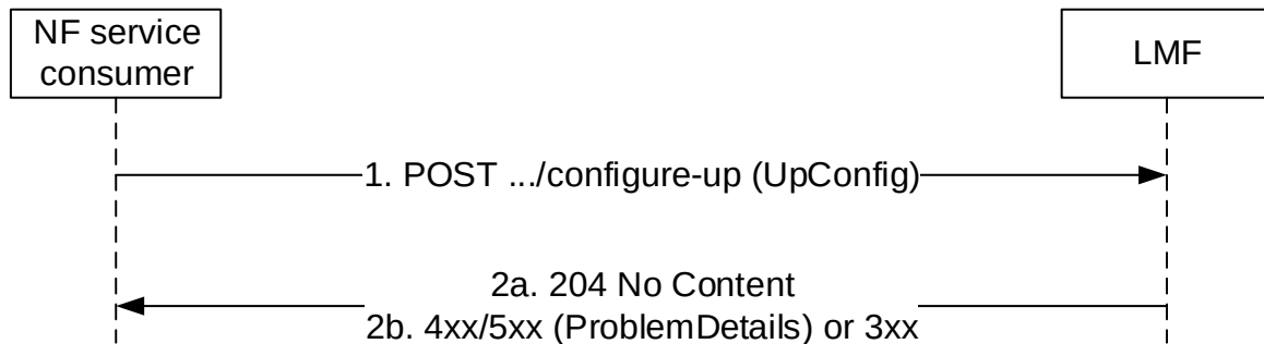
Figure 5.2.2.9.2-1: LCS-UP connection
