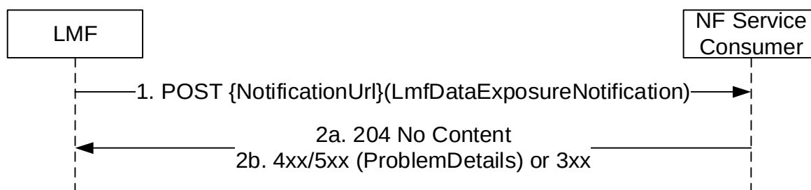
Figure 5.4.2.4-1: Notification for LMF data exposure
