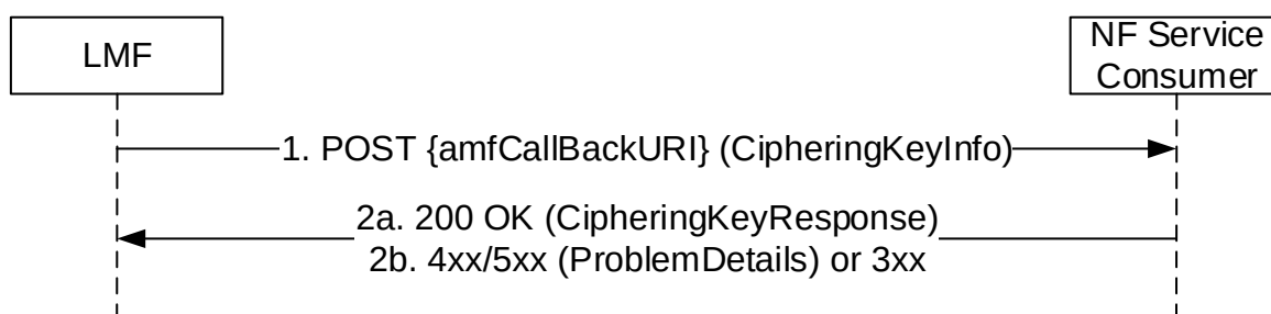
Figure 5.3.2.2.3-1: CipheringKeyData Notify
