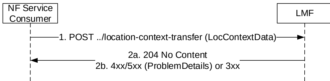
Figure 5.2.2.5.2-1: LocationContextTransfer Request
