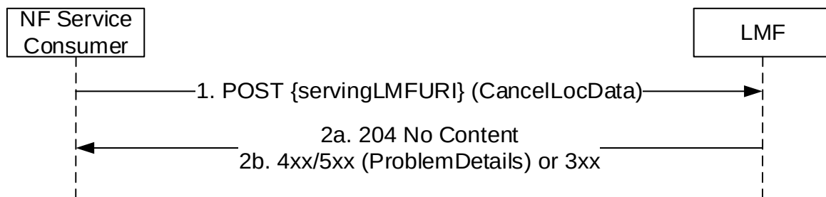
Figure 5.2.2.4.2-1: CancelLocation Request
