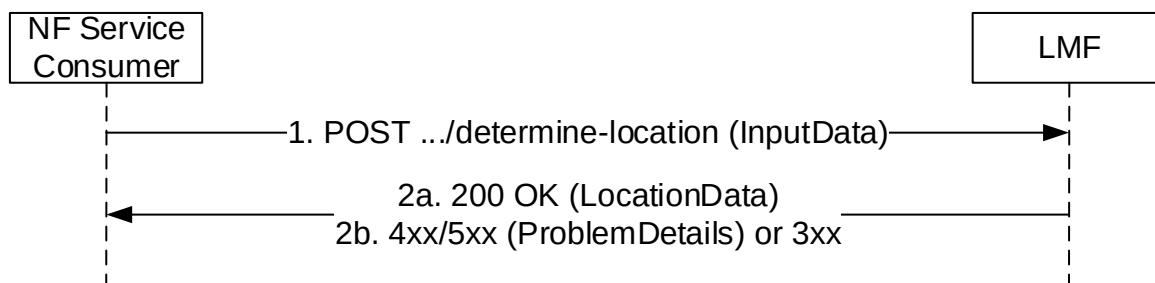
Figure 5.2.2.2-1: DetermineLocation Request
