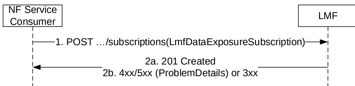
Figure 5.4.2.2-1: Subscription of NF service consumer to LMF data exposure
