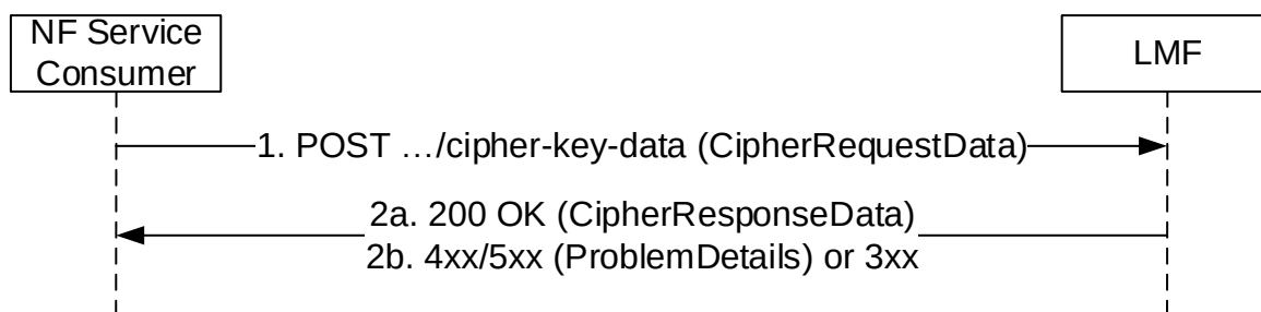
Figure 5.3.2.2-1: CipheringKeyData Request
