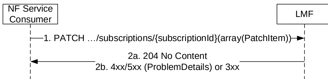
Figure 5.4.2.3-1: Modification of subscription for LMF data exposure
