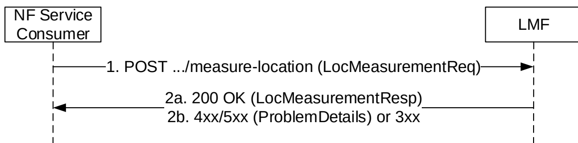
Figure 5.2.2.6.2-1: LocationMeasure Request
