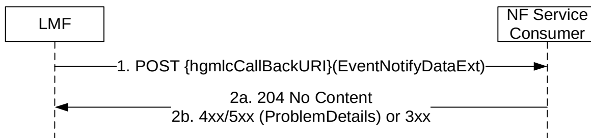
Figure 5.2.2.3.2-1: EventNotify Request
