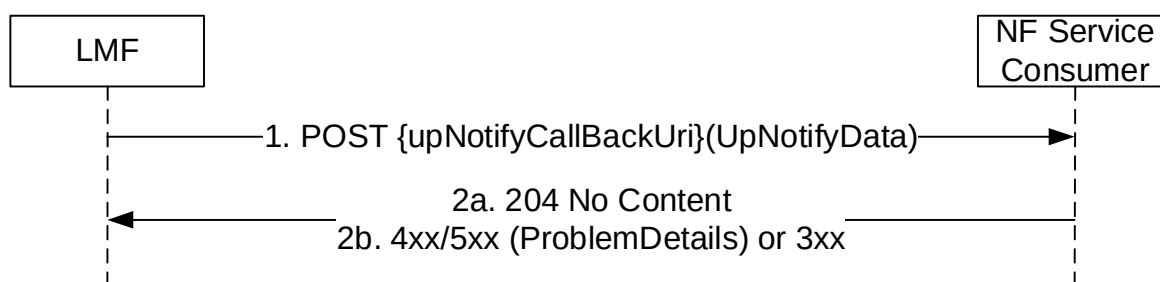
Figure 5.2.2.8.2-1: UPNotify
