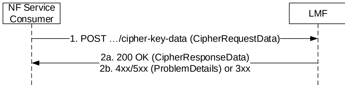
Figure 5.3.2.2-1: CipheringKeyData Request
