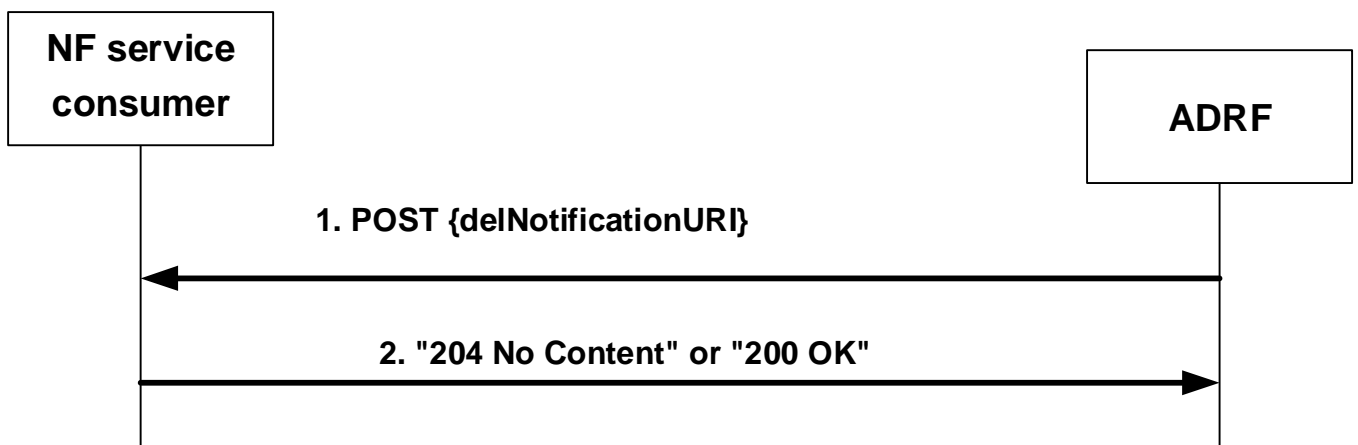
Figure 4.2.2.8.3-1: ADRF notifies the NF service consumer about data or analytics that are about to be deleted.
