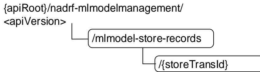
Figure 5.2.3.1-1: Resource URI structure of the Ndrf_MLModelManagement API
