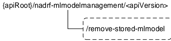
Figure 5.2.4.1-1: Custom operation URI structure of the NadrflMLModelManagement API
