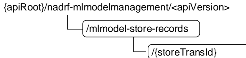
Figure 5.2.3.1-1: Resource URI structure of the Nadrif_MLModelManagement API
