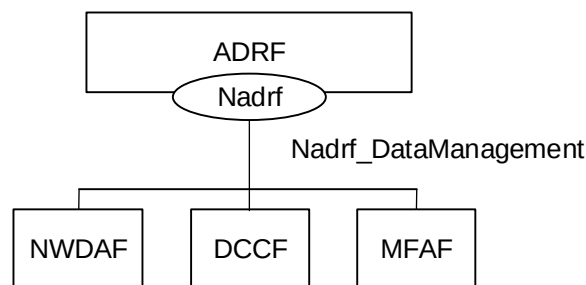
Figure 4.2.1.2-1: Reference Architecture for the Nadrf_DataManagement Service; SBI representation
